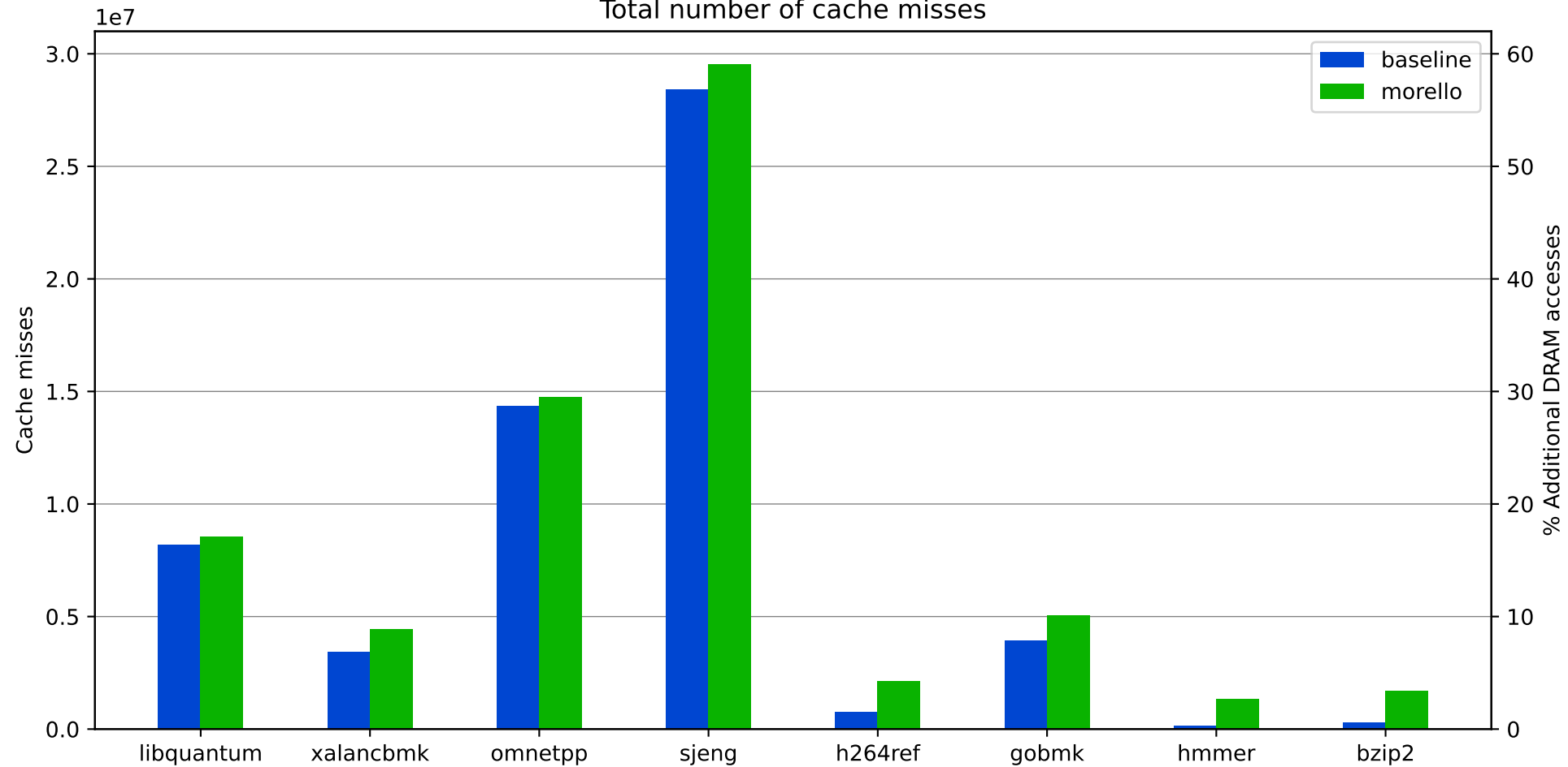
Total number of cache misses
