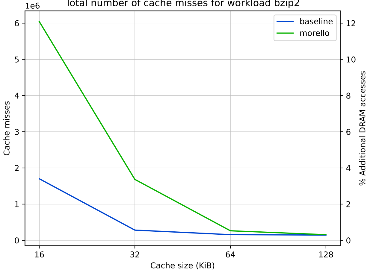
Total number of cache misses for workload bzip2
