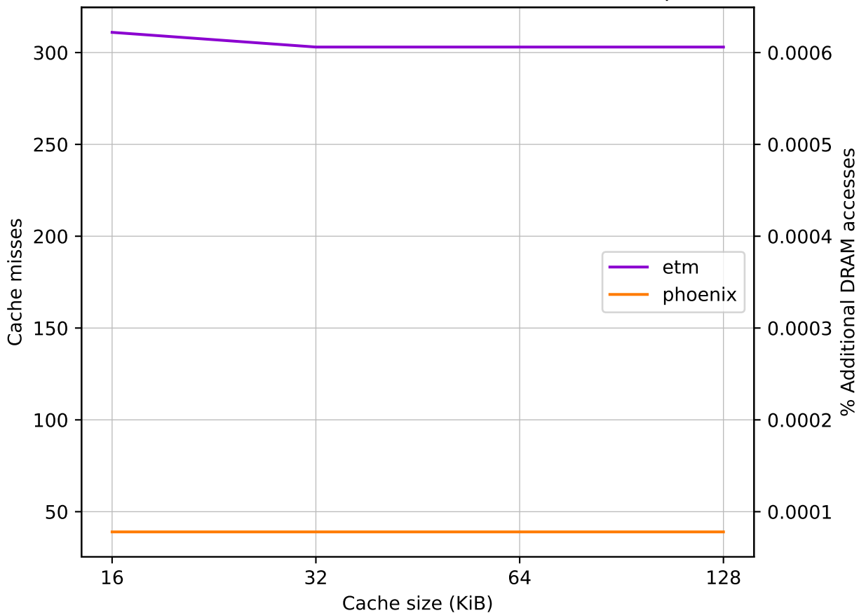
Total number of cache misses for workload bzip2
