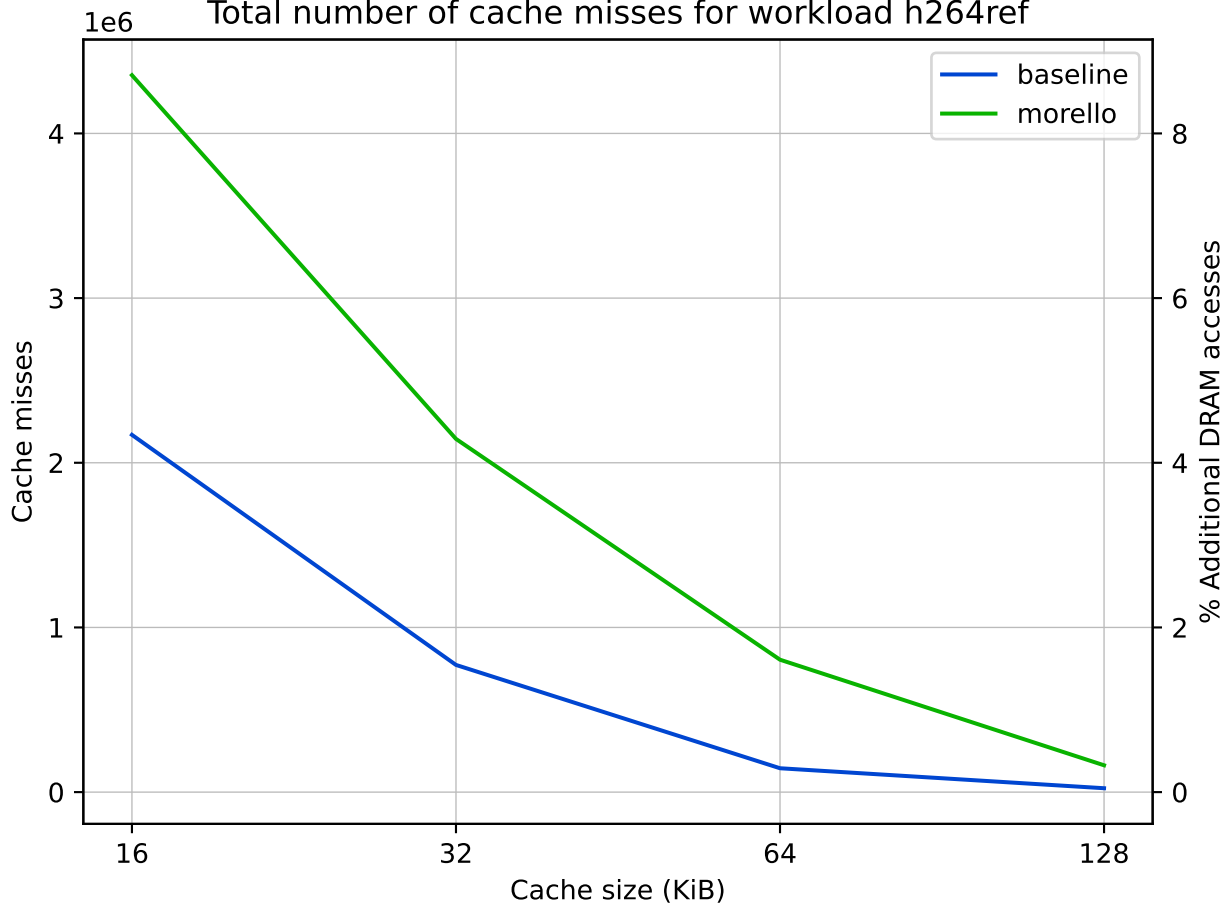
Total number of cache misses for workload h264ref
