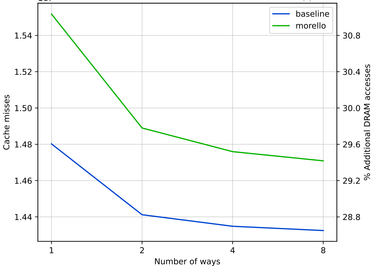
1e7 Total number of cache misses for workload omnetpp
