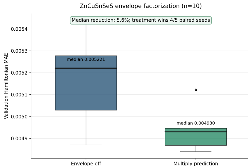
Figure 5: Results for the ZnCuSnSeS envelope-factorization ablation. The two boxplots summarize the final W&B validation Hamiltonian MAE across seeds; black horizontal marks denote medians. The fitted envelope reduces the median error by 5.6% and wins four of five paired runs.
