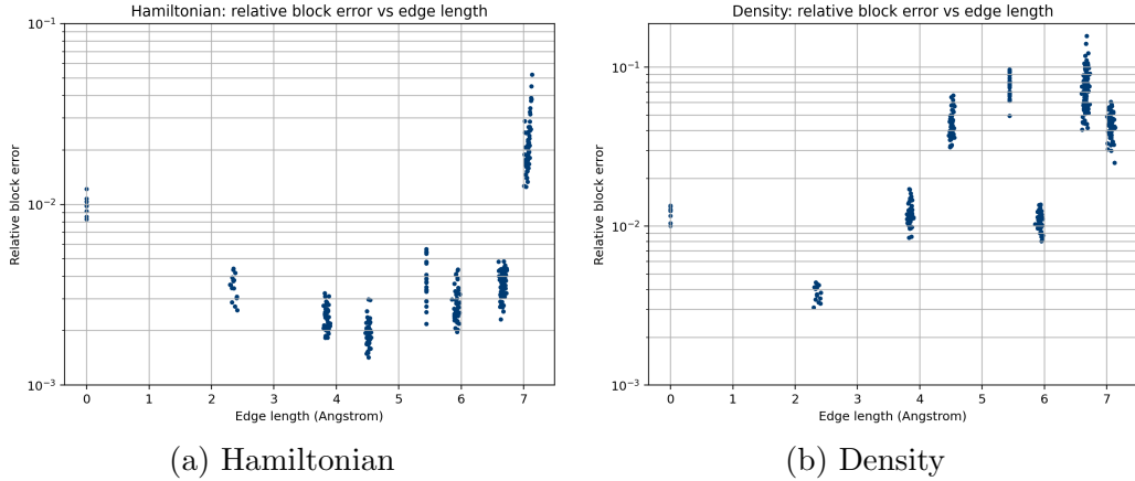
Figure 10: Relative block error by atom-pair distance for the representative perturbed-silicon structure. Each point is one shift-resolved block. Both axes span at least 10^{-3} to 10^{-1} to permit a direct comparison of the two matrix targets.
