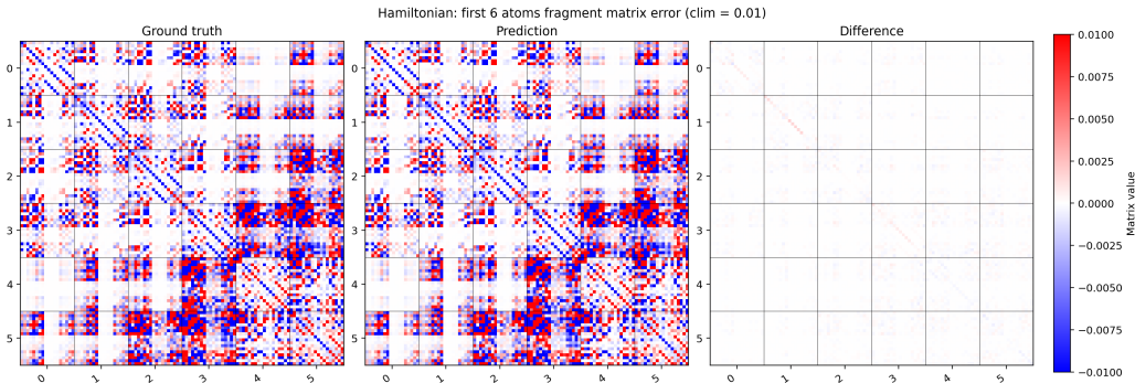
Figure 5: Reference, predicted, and residual Hamiltonian fragments for the first six atoms of a held-out \text{ZnCuSnSeS} validation structure. The common color range is \pm 0.01 eV.
