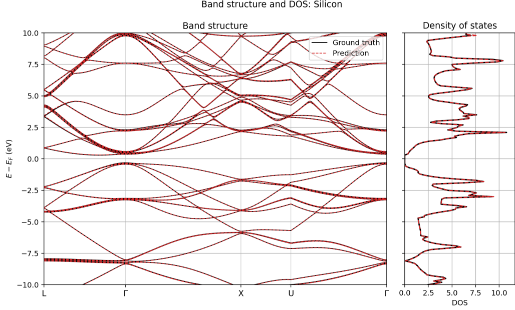
Figure 8: Band structure and density of states for a held-out perturbed-silicon validation structure. Reference values are black solid lines and predictions are red dashed lines. The DOS is integrated using a 4 \times 4 \times 4 tetrahedron mesh.
