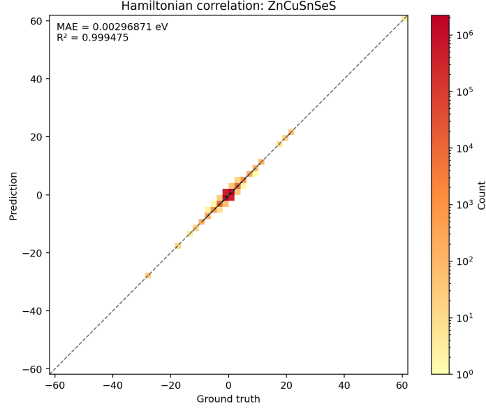
Figure 6: Element-wise Hamiltonian correlation for the same ZnCuSnSeS structure. The heat map shows bin counts on a logarithmic scale, black points overlay all matrix elements, and the dashed line denotes equality.
