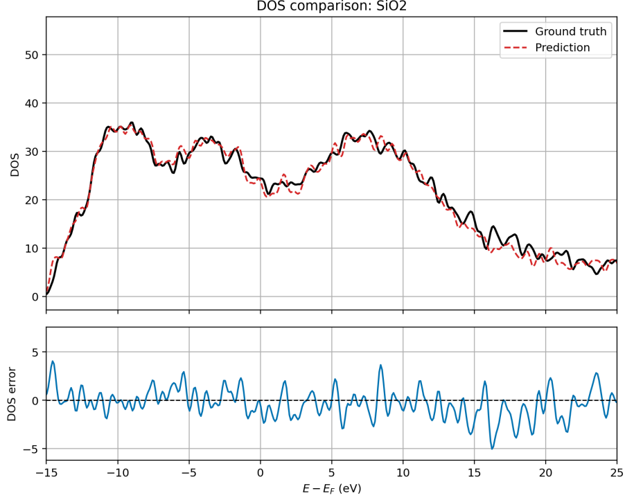
Figure 7: Reference and predicted density of states for a held-out \text{SiO}_2 validation structure (top), together with their difference (bottom). Energies are referenced to the respective Fermi levels. The calculation uses Gaussian broadening with \sigma = 0.2 eV on a 2 \times 2 \times 2 mesh.
