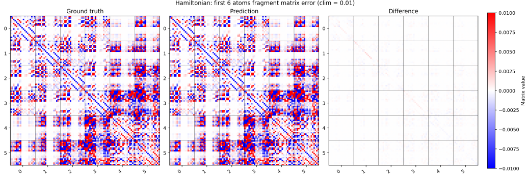
Figure 5: Hamiltonian fragments for the first six atoms of a representative \text{ZnCu}_2\text{Sn}(\text{SeS})_2 validation structure. The common color range is \pm 0.01 eV, and periodic-image contributions remain shift-resolved.
