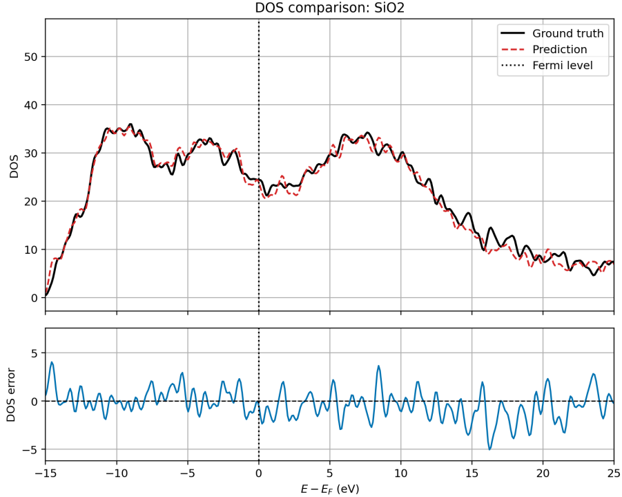
Figure 7: Density of states and its prediction error for a representative glassy \text{SiO}_2 validation structure. The calculation uses Gaussian broadening with \sigma = 0.2 eV on a 2 \times 2 \times 2 k-point mesh. The dotted line marks the Fermi level.
