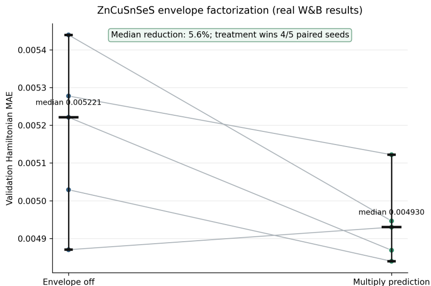
Figure 5: Real results for the ZnCuSnSeS envelope-factorization ablation. Colored points show the final W&B validation Hamiltonian MAE for seeds 41–45, and gray lines connect paired seeds. Horizontal black marks denote medians; vertical black intervals are percentile bootstrap intervals for the median. The fitted envelope reduces the median error by 5.6% and wins four of five paired runs.
