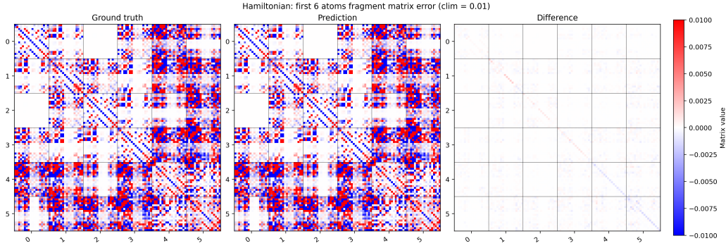
Figure 7: Hamiltonian fragments for the first six atoms of a representative \text{ZnCu}_2\text{Sn}(\text{SeS})_2 validation structure. The common color range is \pm 0.01 eV.
