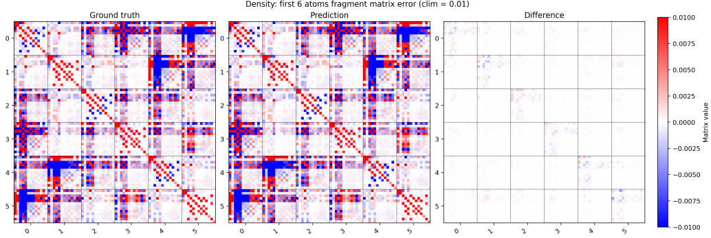
Figure 9: Reference, predicted, and residual density-matrix fragments for the first six atoms of the perturbed-silicon validation structure. The common color range is \pm 0.01 in the native density-matrix units.
