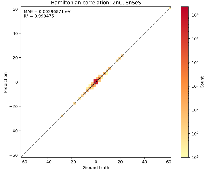
Figure 6: Element-wise Hamiltonian correlation for the same ZnCuSnSeS structure. The heat map shows bin counts on a logarithmic scale, black points overlay all matrix elements, and the dashed line denotes equality. The element-weighted, shift-resolved MAE is 0.002969 eV.
