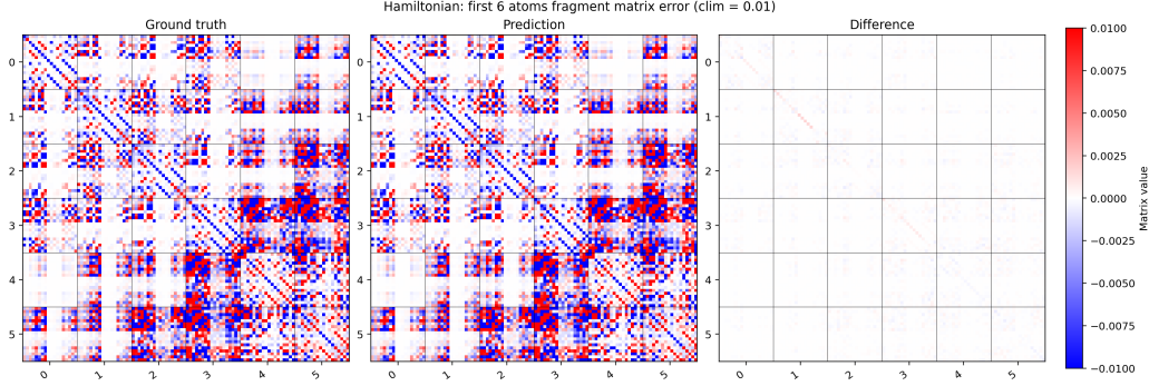
Figure 5: Reference, predicted, and residual Hamiltonian fragments for the first six atoms of a held-out ZnCuSnSeS validation structure. The common color range is \pm 0.01 eV. Blocks retain their real-space lattice-shift resolution; they are not collapsed to a \Gamma -point matrix.
