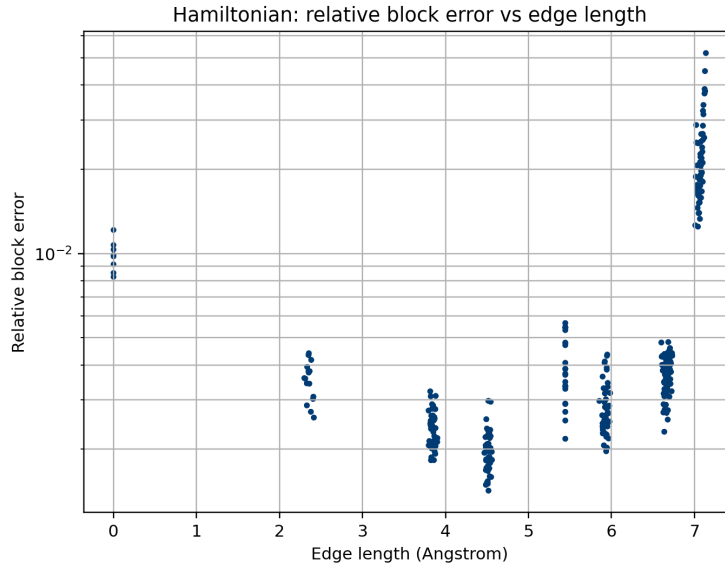
Figure 10: Relative Hamiltonian block error as a function of atom-pair edge length for the same perturbed-silicon structure. Each point represents one shift-resolved atom-pair block.
