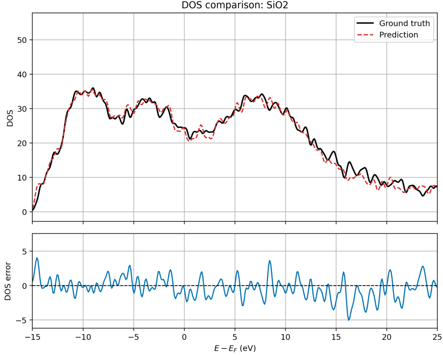
Figure 7: Reference and predicted density of states for a held-out \text{SiO}_2 validation structure (top), together with their signed difference (bottom). Energies are referenced to the respective Fermi levels. The calculation uses Gaussian broadening with \sigma = 0.2 eV on a 2 \times 2 \times 2 mesh.
