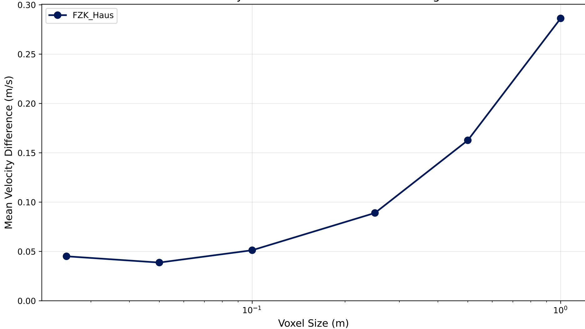
Mean Velocity Difference vs Voxel Size - 45 Degrees
