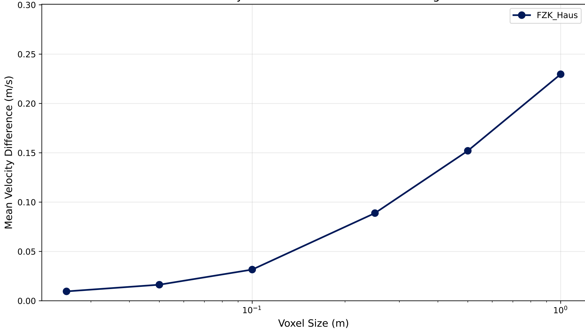
Mean Velocity Difference vs Voxel Size - 90 Degrees
