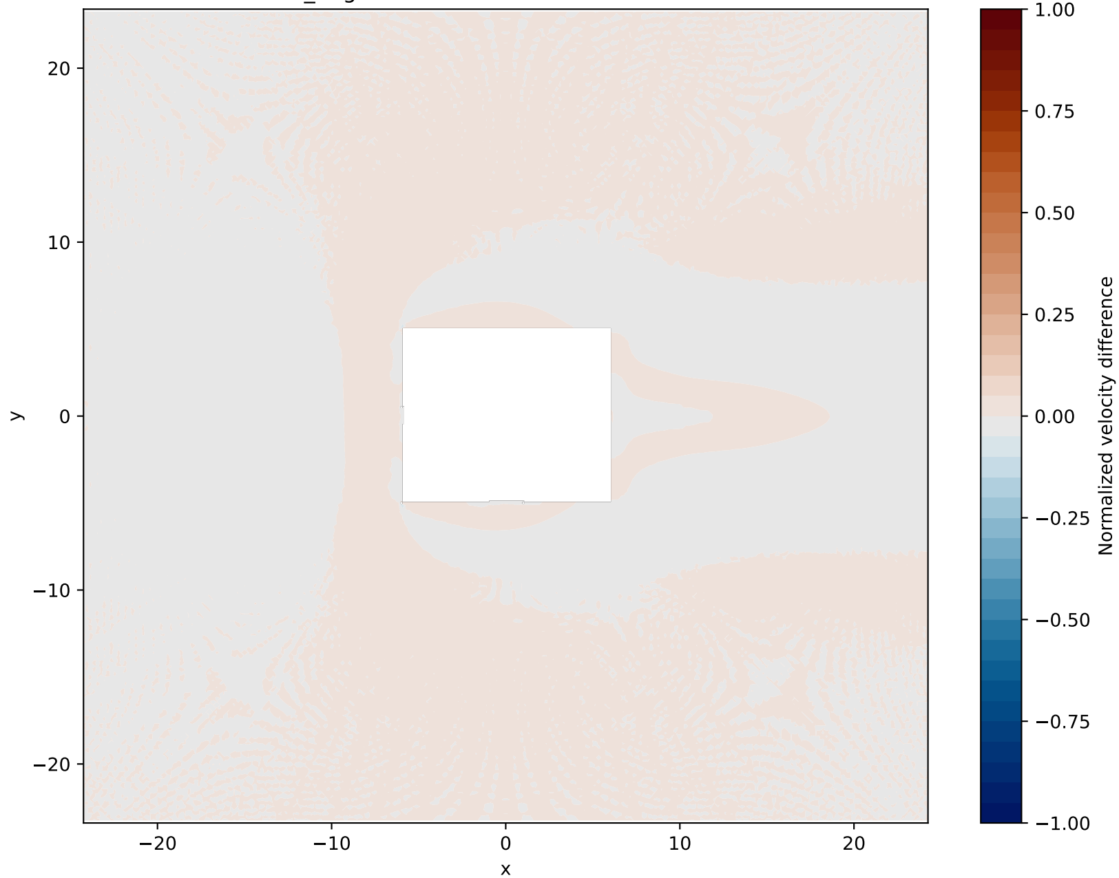
360_degrees - 0025m error at z=0.5390625
