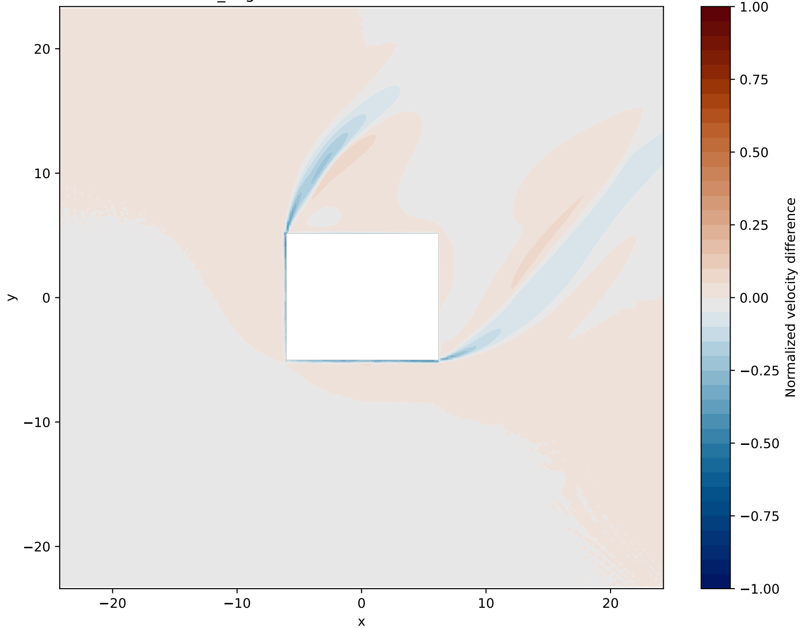
45_degrees - 025m error at z=0.5390625
