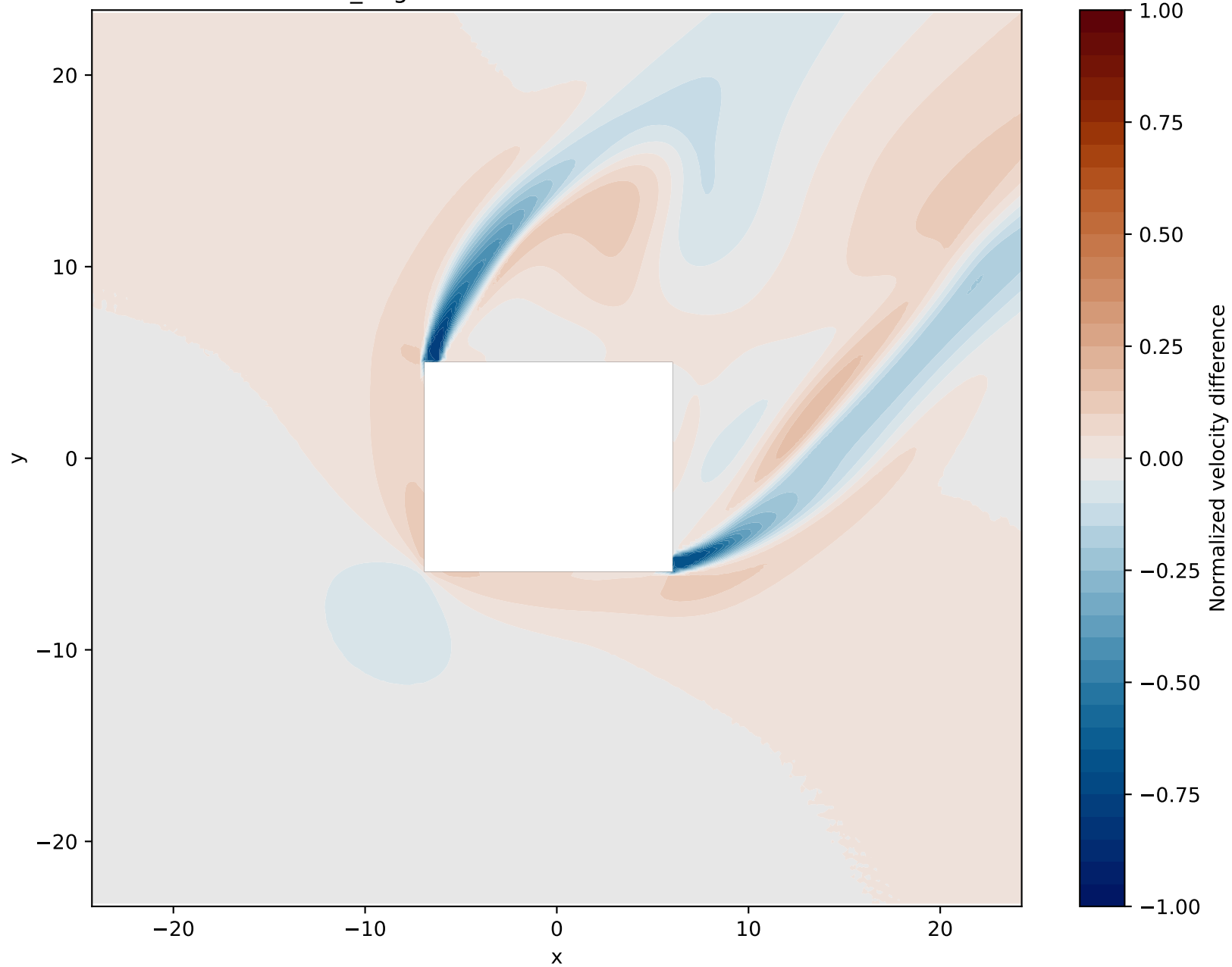
45_degrees - 1m error at z=0.5390625
