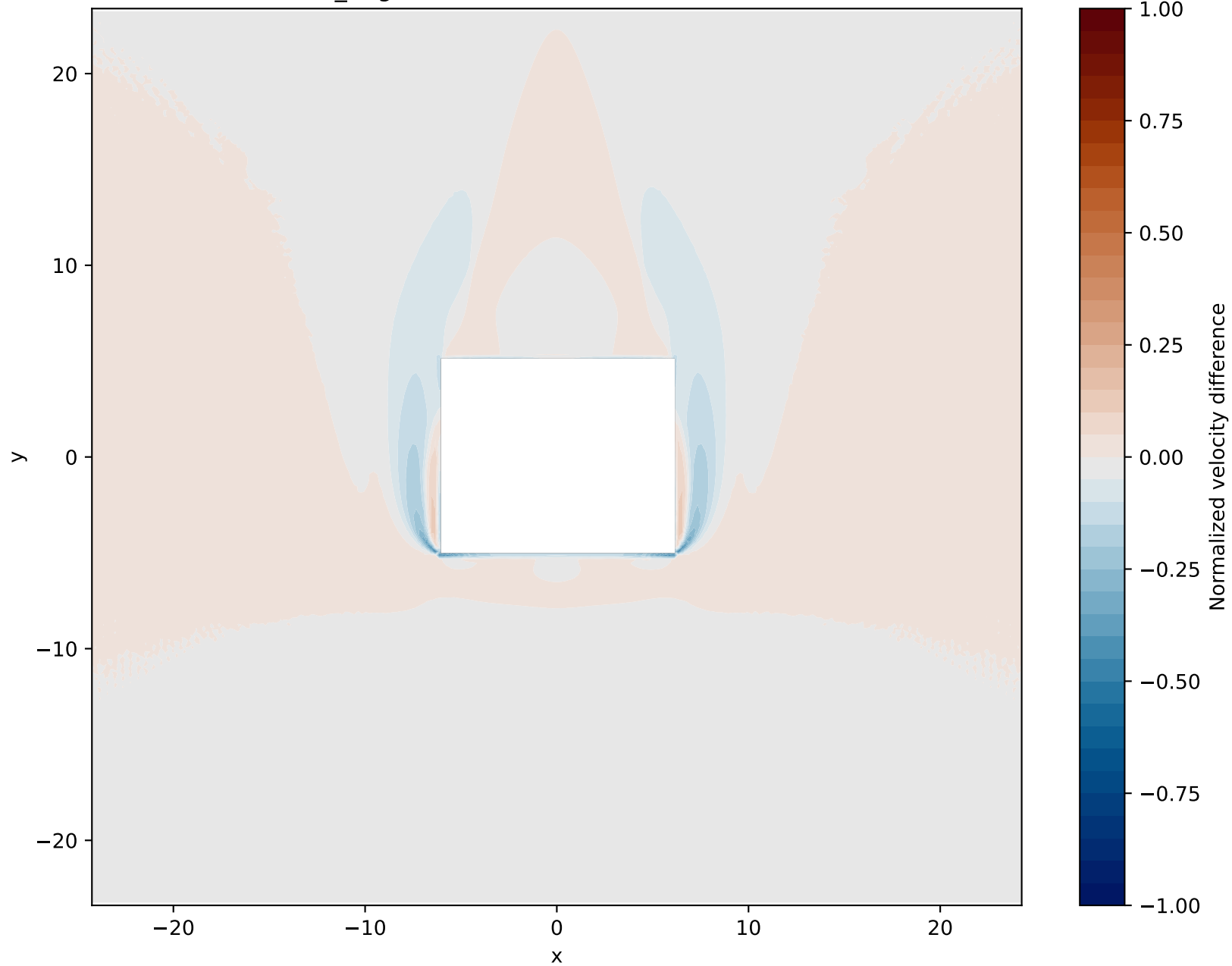
90_degrees - 025m error at z=0.5390625
