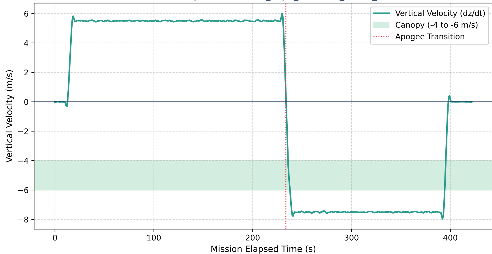
Vertical Velocity Profile — 02_high_altitude_burst_1200m
