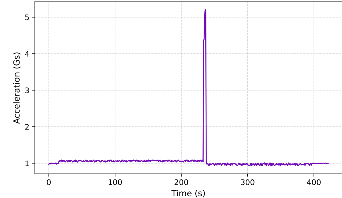
C. G-Shock (Peak: 5.21G)
