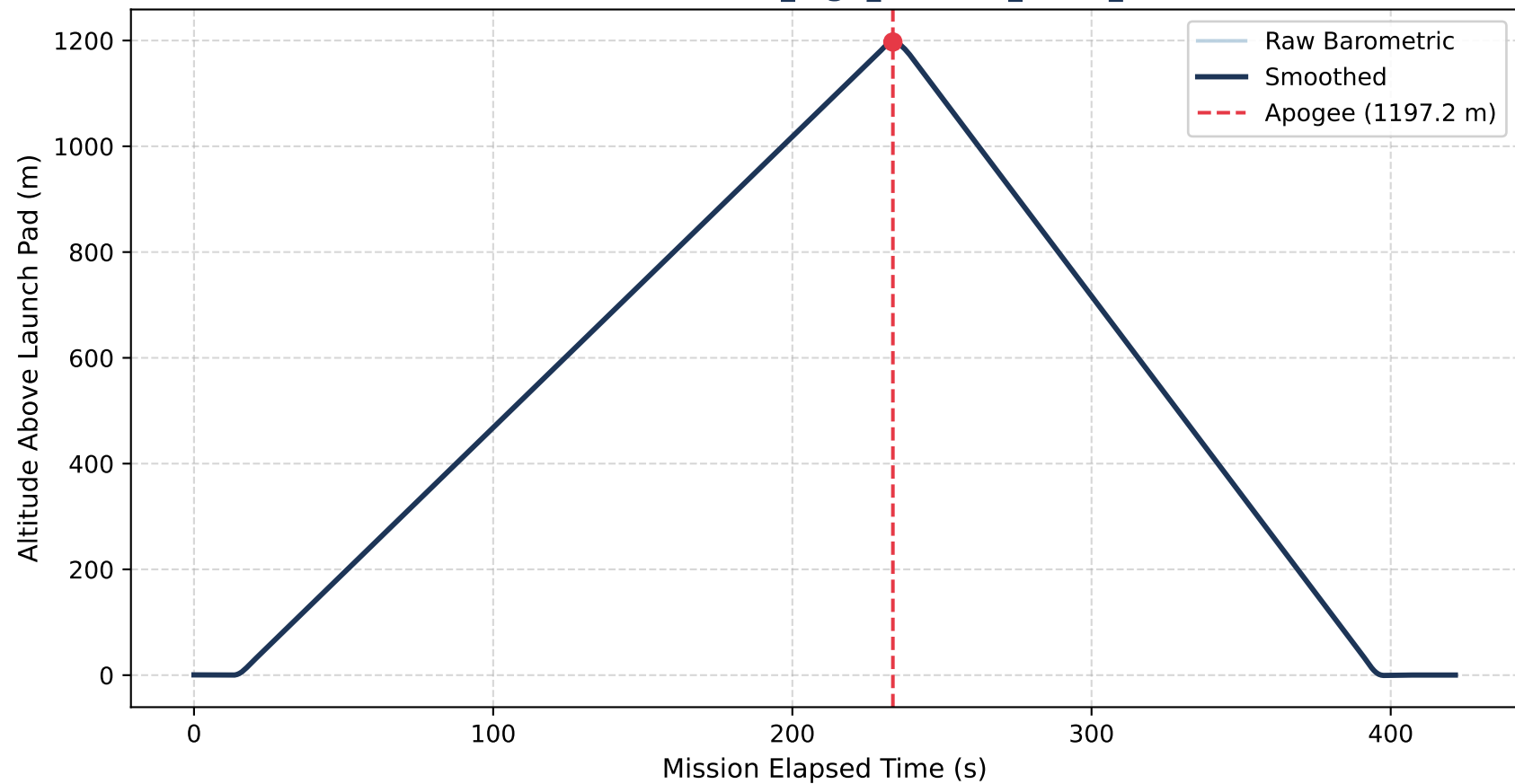
Altitude vs. Time — 02_high_altitude_burst_1200m
