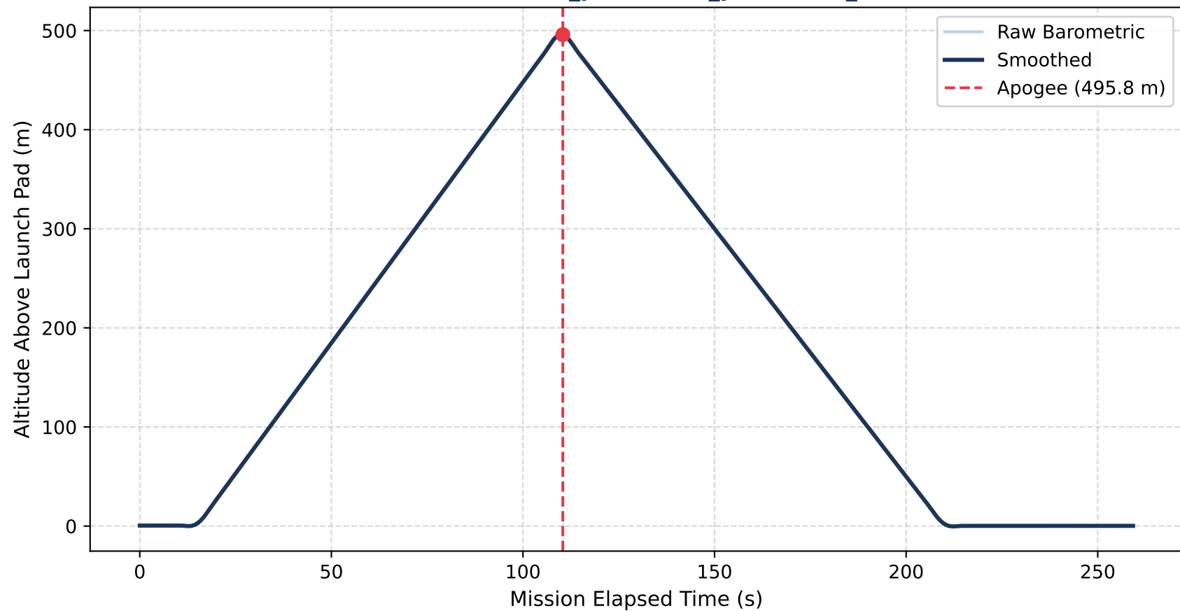
Altitude vs. Time — 05_parachute_pendulum_resonance
