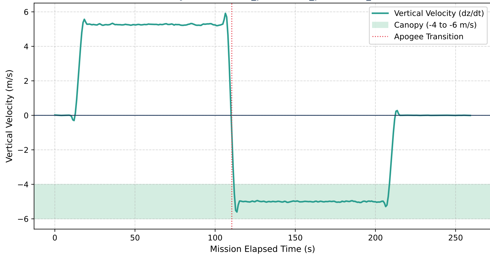
Vertical Velocity Profile — 05_parachute_pendulum_resonance
