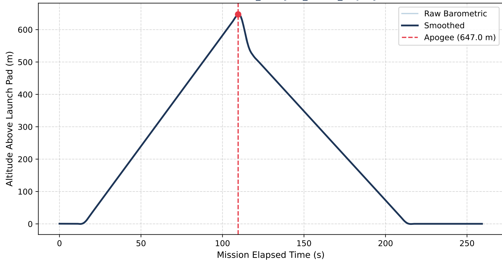
Altitude vs. Time — 06_delayed_chute_deployment
