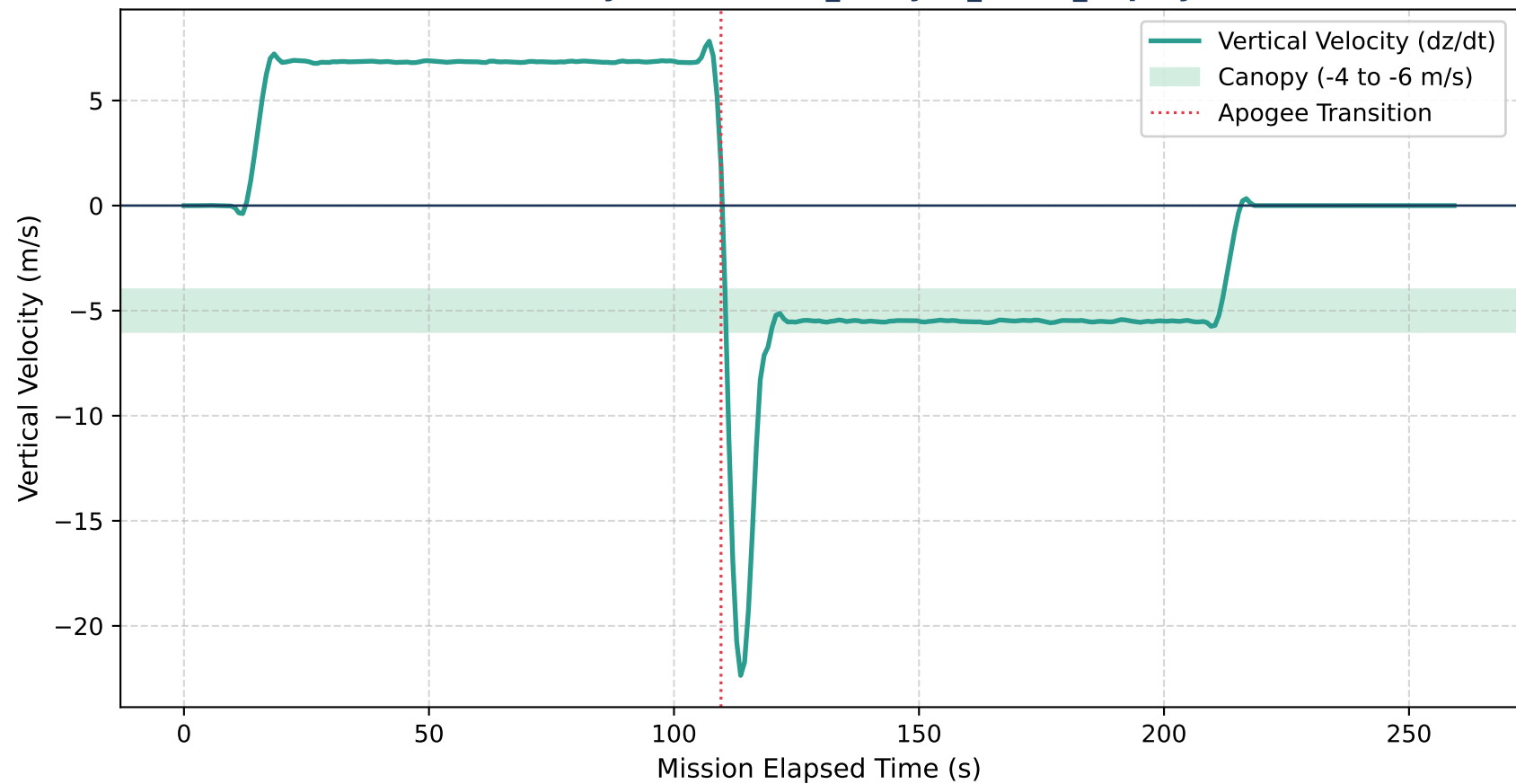
Vertical Velocity Profile — 06_delayed_chute_deployment
