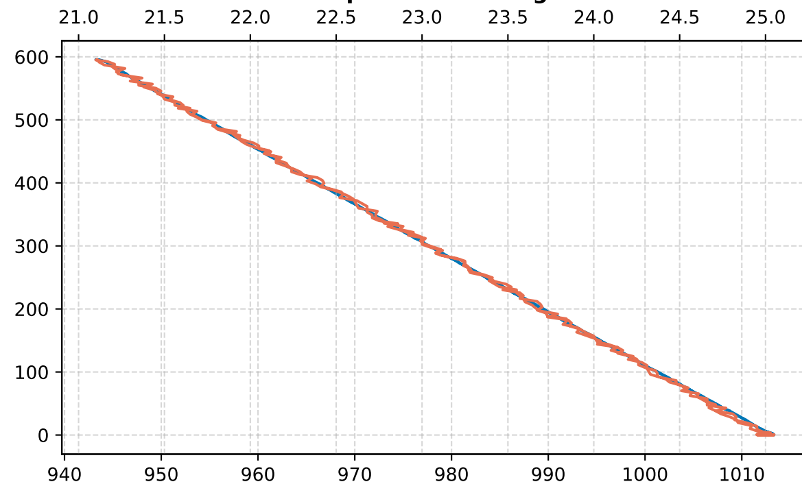
D. Atmospheric Sounding Profile
