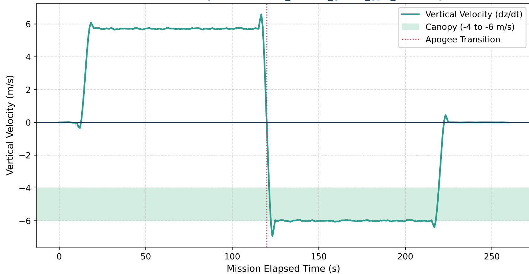
Vertical Velocity Profile — 08_sensor_glitch_gps_recovery
