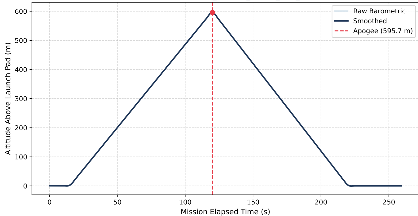
Altitude vs. Time — 08_sensor_glitch_gps_recovery
