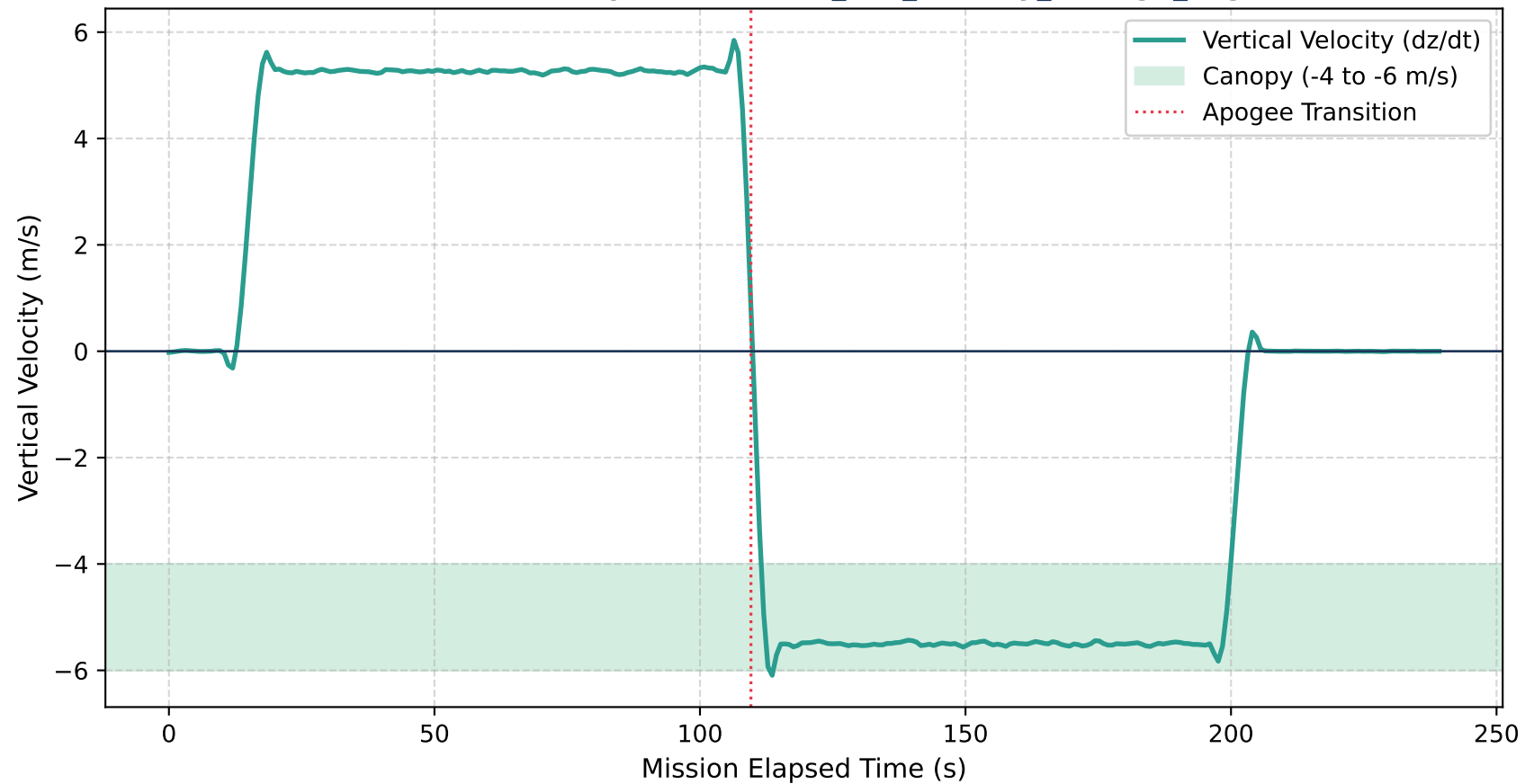
Vertical Velocity Profile — 09_low_battery_voltage_sag
