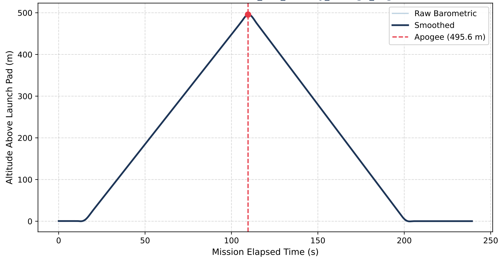
Altitude vs. Time — 09_low_battery_voltage_sag
