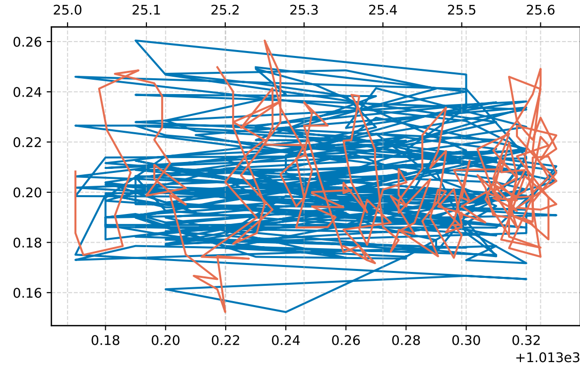
D. Atmospheric Sounding Profile
