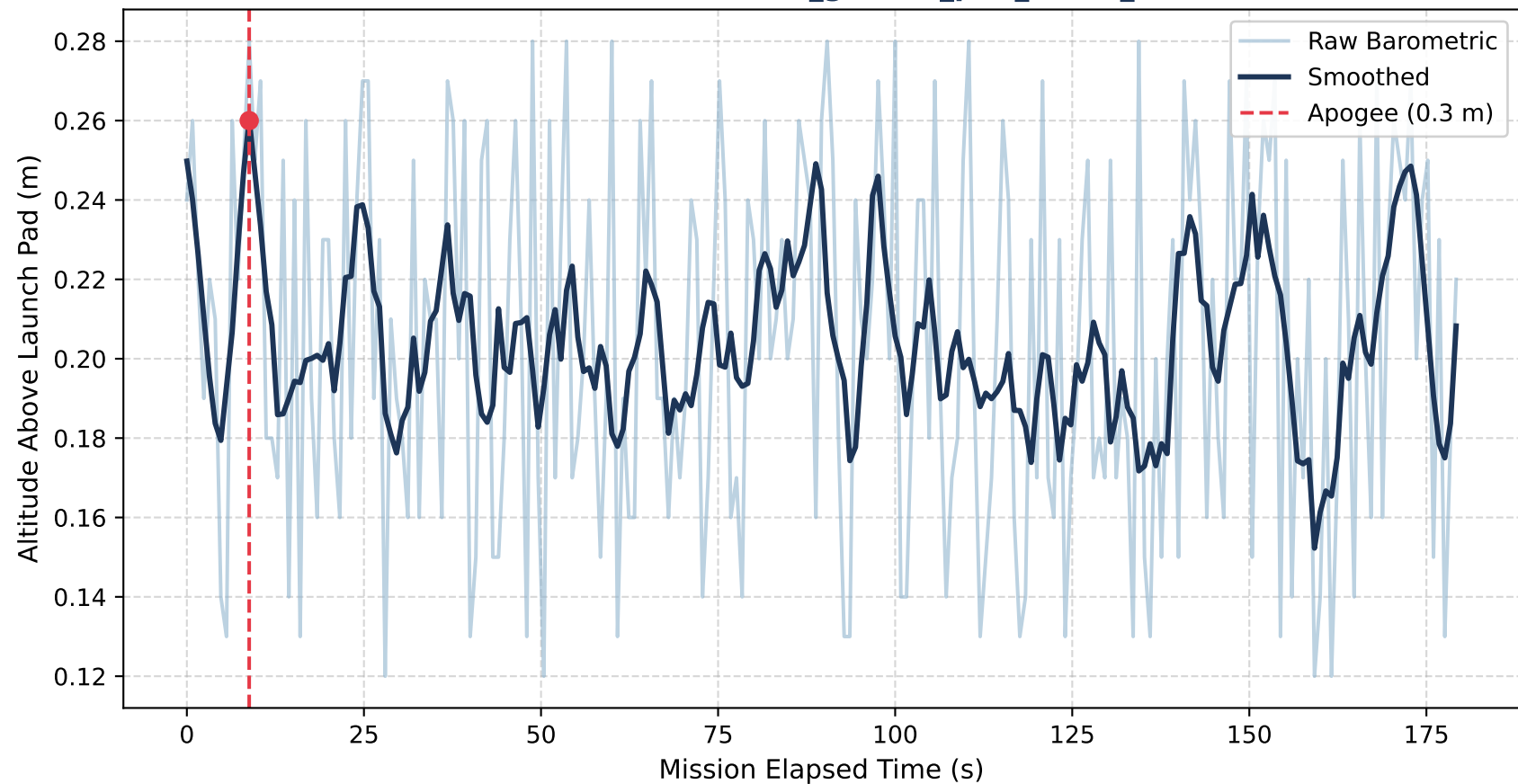
Altitude vs. Time — 10_ground_pad_static_test
