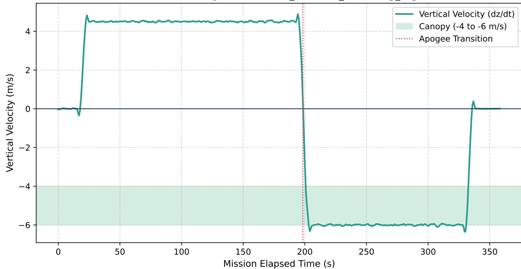
Vertical Velocity Profile — 01_nominal_sounding_flight
