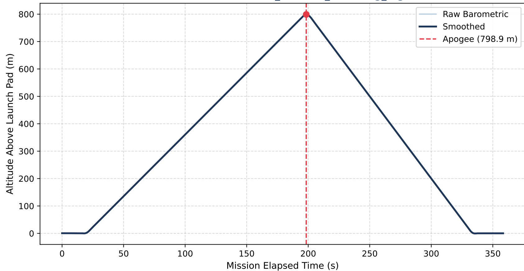
Altitude vs. Time — 01_nominal_sounding_flight
