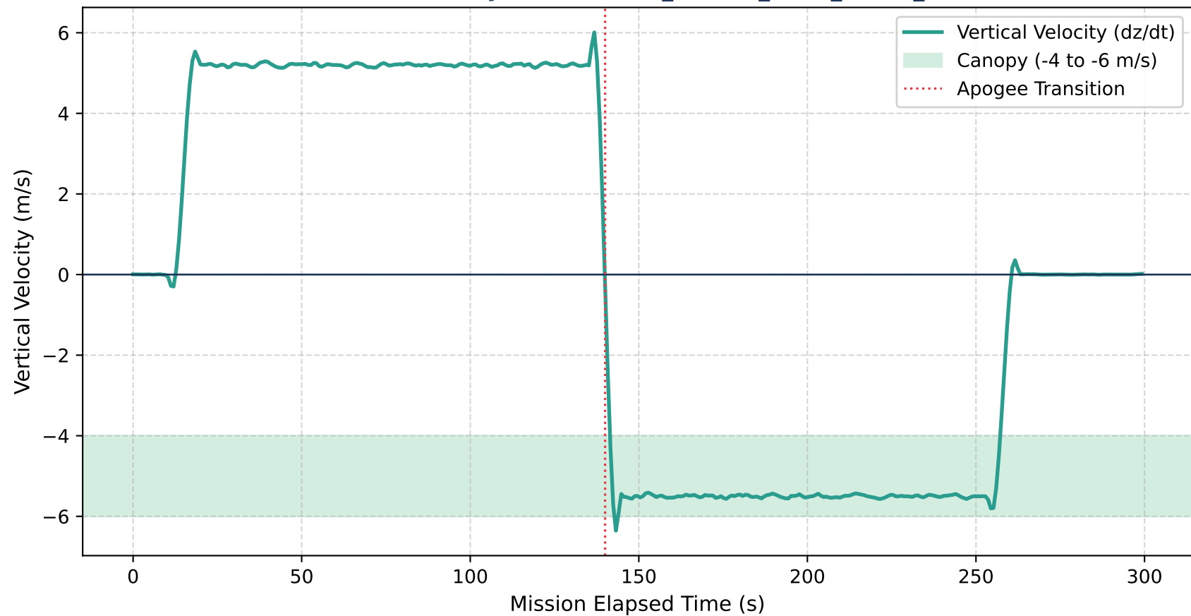
Vertical Velocity Profile — 03_severe_wind_shear_drift
