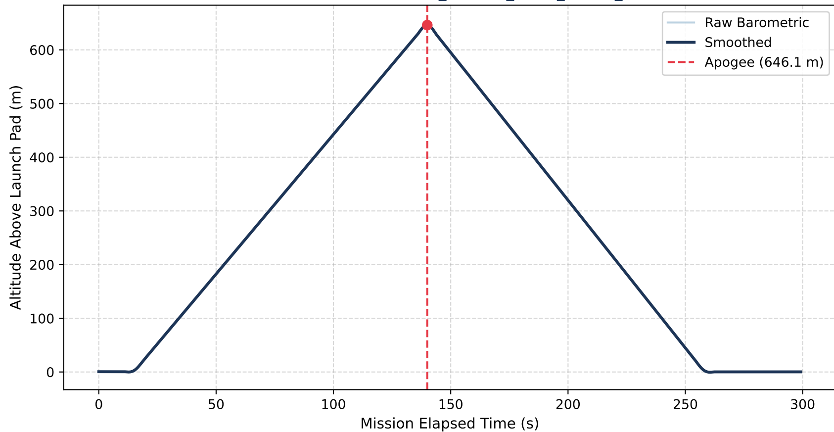
Altitude vs. Time — 03_severe_wind_shear_drift
