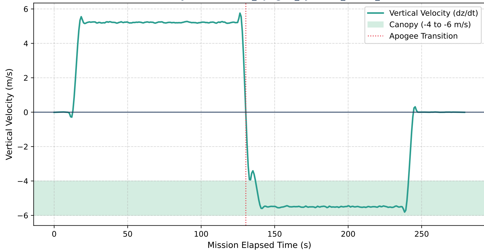
Vertical Velocity Profile — 04_apogee_ejection_shock_tumble
