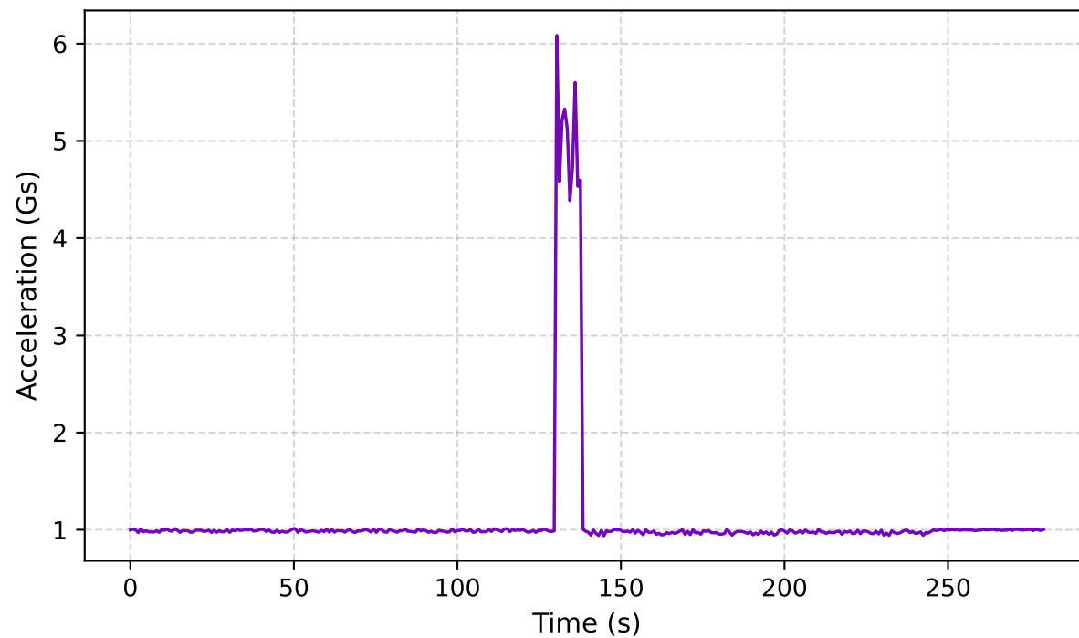
C. G-Shock (Peak: 6.08G)
