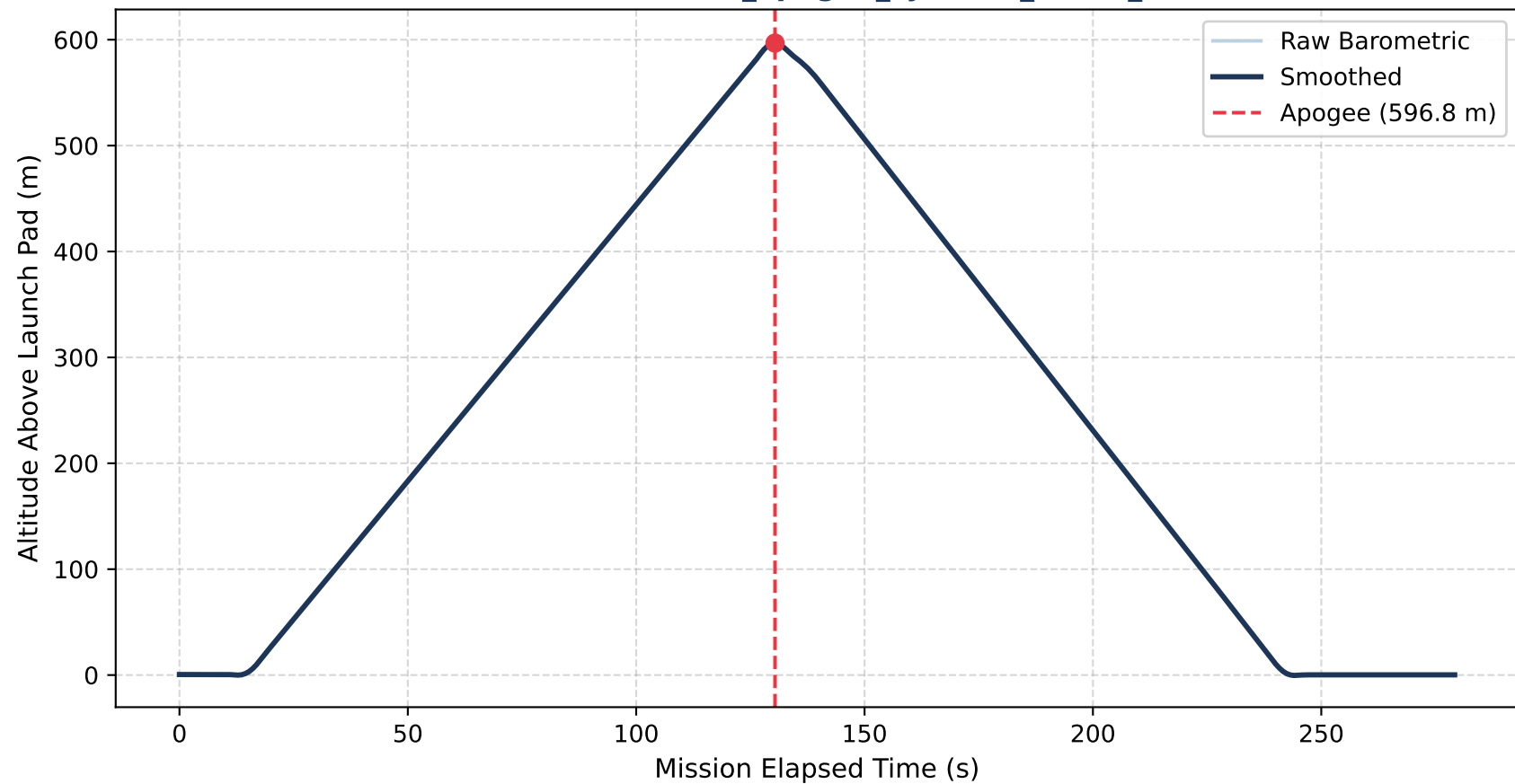
Altitude vs. Time — 04_apogee_ejection_shock_tumble
