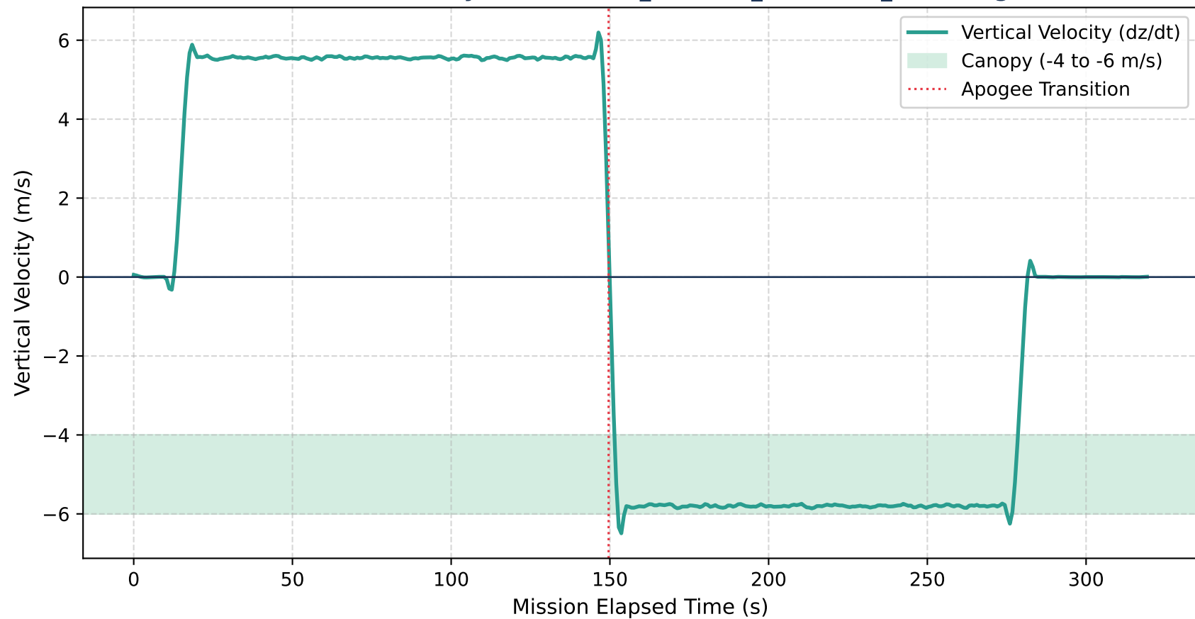
Vertical Velocity Profile — 07_thermal_inversion_sounding
