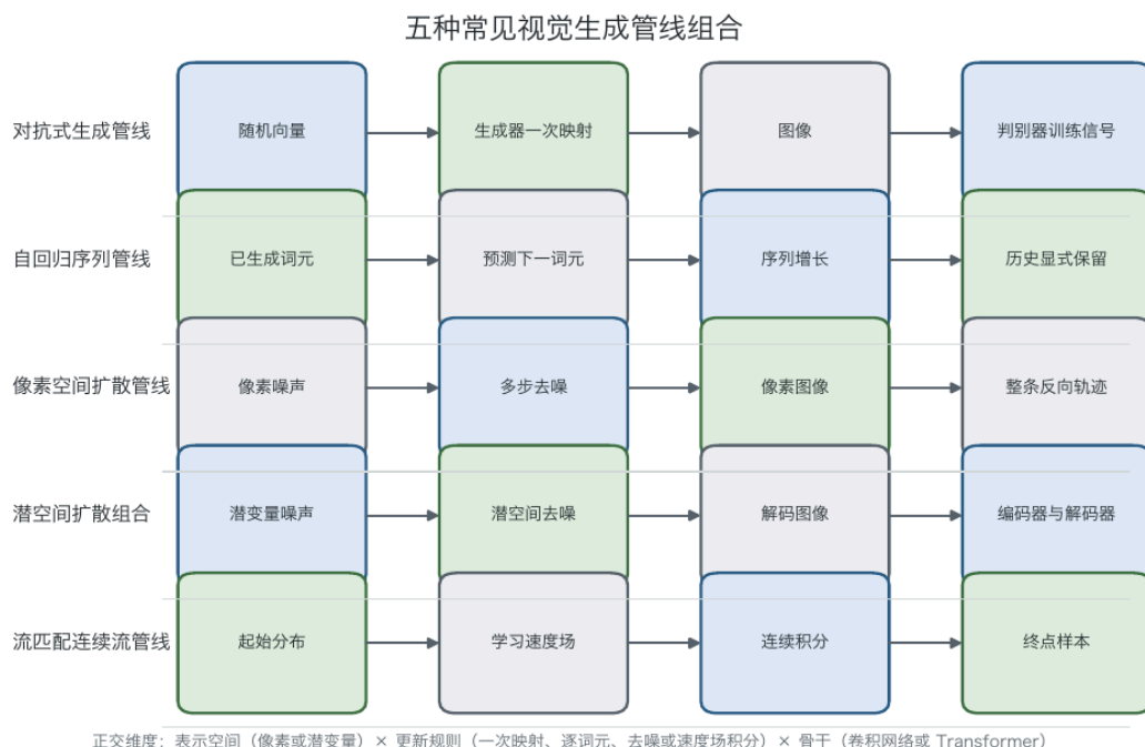
Five swimlanes compare common pipeline combinations such as adversarial generation, autoregressive sequences, pixel-space diffusion, latent-space diffusion, and flow-matching continuous flow, and list the three orthogonal dimensions of representation space, update rule, and model backbone at the bottom.
