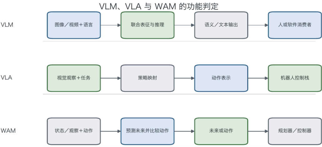
Three swimlanes list the inputs, mechanisms, outputs, and consumers of the vision–language model, the vision–language–action model, and the world action model.
