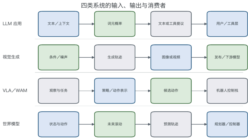
Four horizontal swimlanes showing the input, internal process, output, and consumer of the language model, visual generation, vision-language-action system, and world model, respectively.
