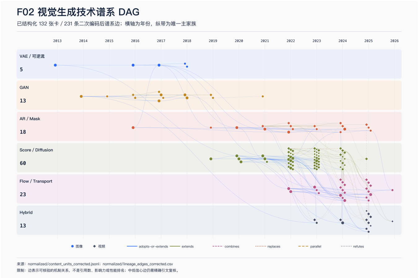
F02. Visual generation technical lineage. The figure fully includes 132 work nodes and 231 edges retained by second-pass encoding. Colors denote the generation-update family of each work, and circles/diamonds denote image/video, respectively. Evidence boundary: edges denote verifiable mechanism relations, not citation counts, influence, or performance rankings. Medium- and low-confidence edges still require precise citation review.
