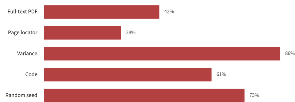
Missingness audit
