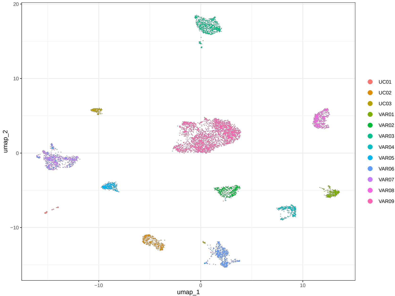
Tumour epithelial audit UMAP: patient
