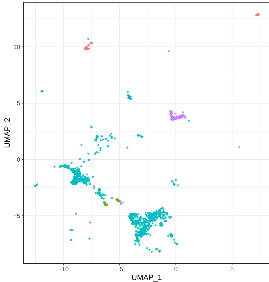
UC01/current 12049: broad annotation
