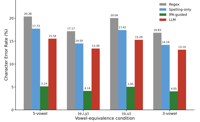
Fig. 2. Overall CER (%) under four vowel-equivalence conditions.
