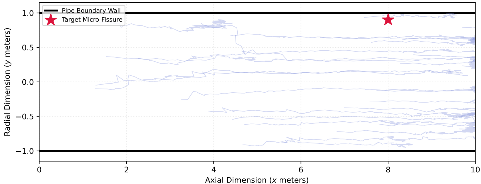
Extreme Stochastic Gamma Field: Path Deviation Under Turbulent Drag (Decentralized M-PSO, all 25 agents, single representative run)
