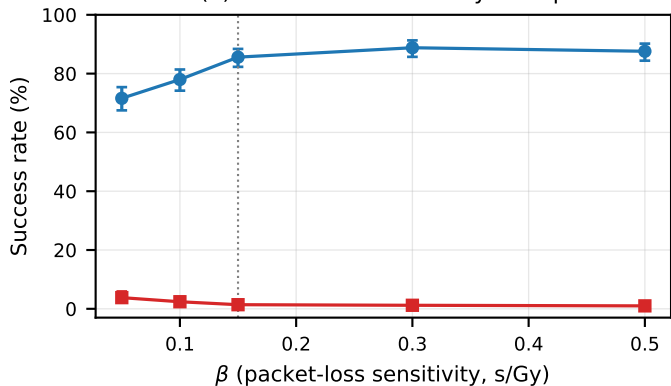
(a) Packet-loss sensitivity sweep
