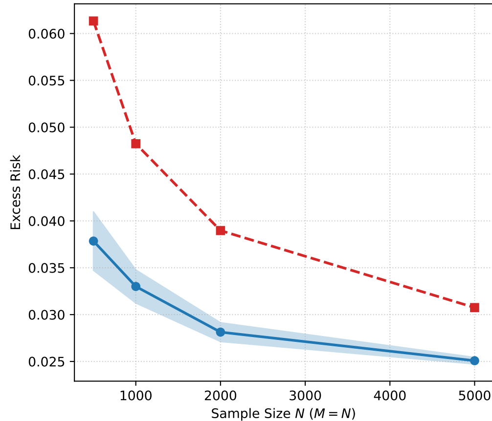
Toy Distribution 3 (Noisy Side Info)
