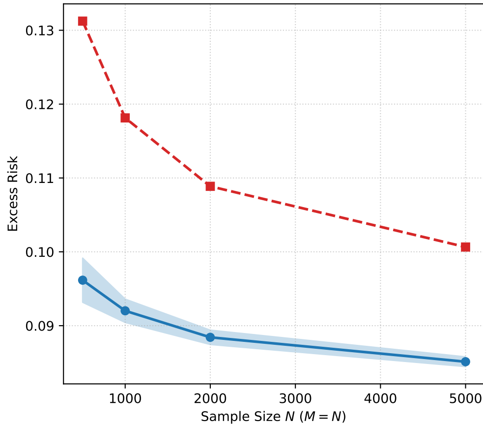
Toy Distribution 2 (Moderate Signal)
