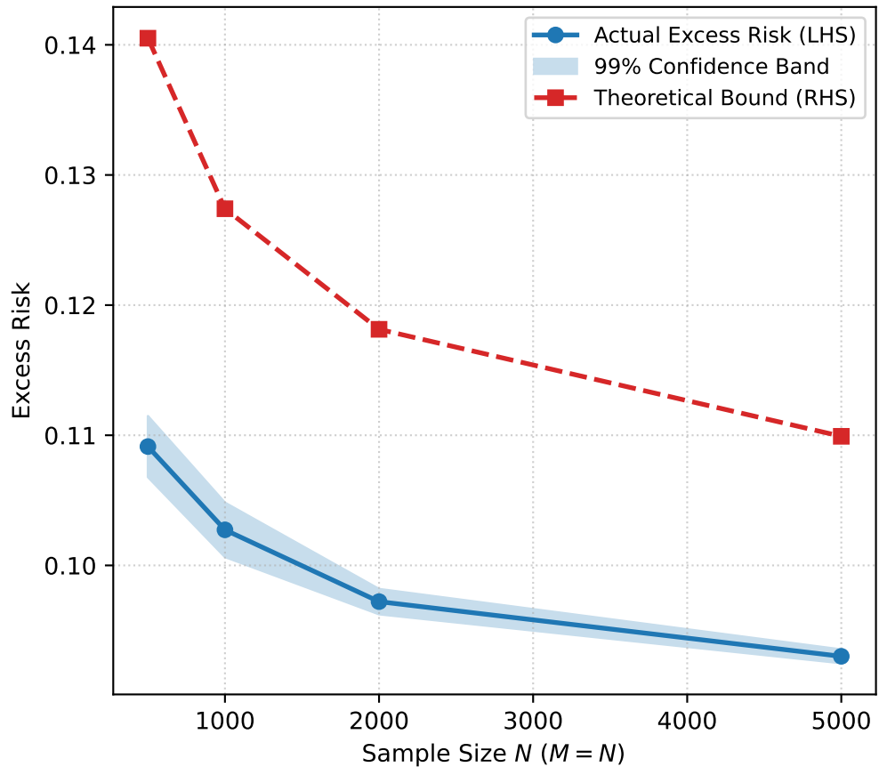
Toy Distribution 1 (High Signal)
