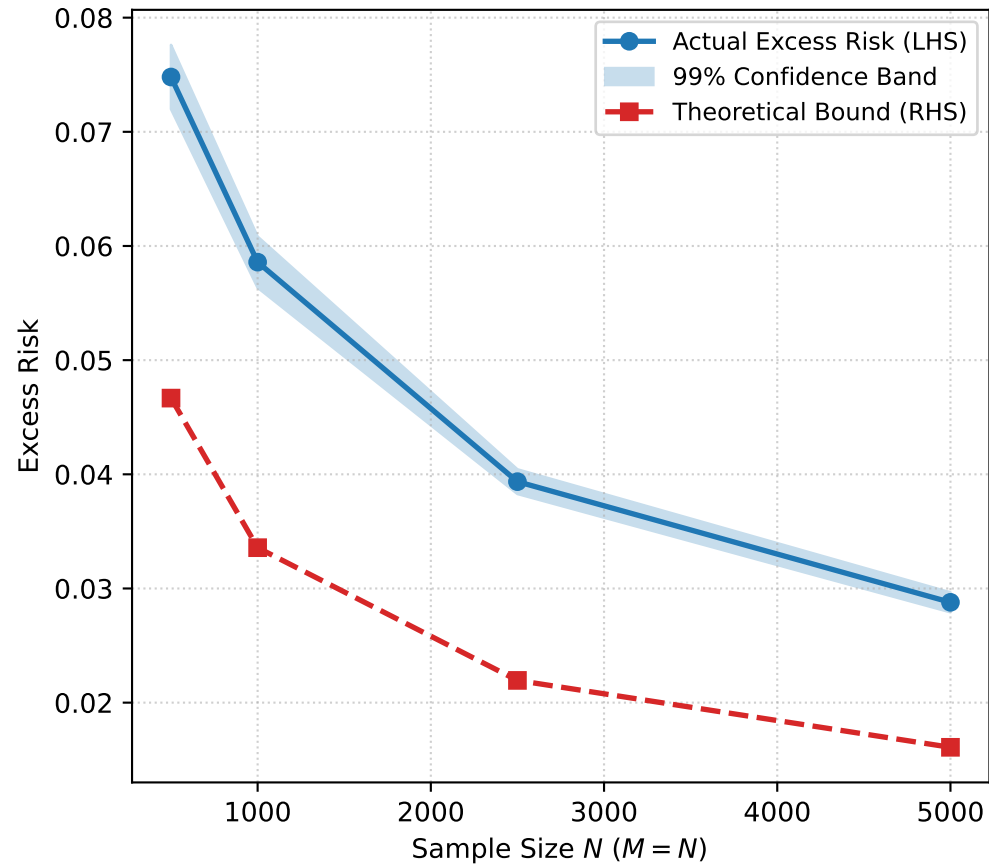
Adult Income
