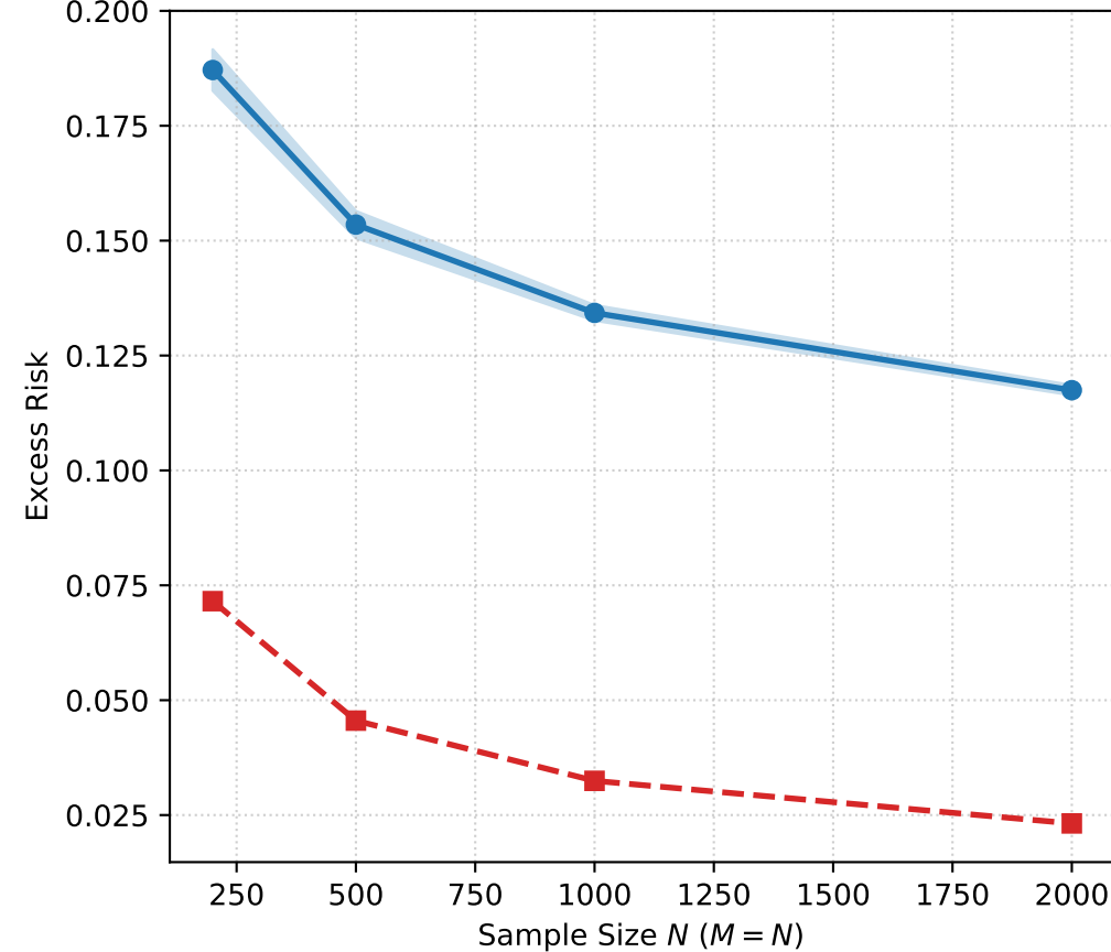
Mushroom
