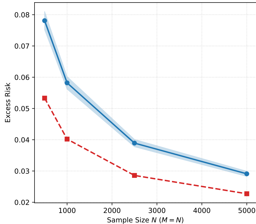
Bank Marketing
