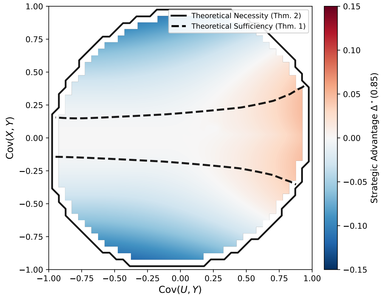
Strategic Advantage at Noise q = 0.85 ( \text{Cov}(X, U) = 0.1 )
