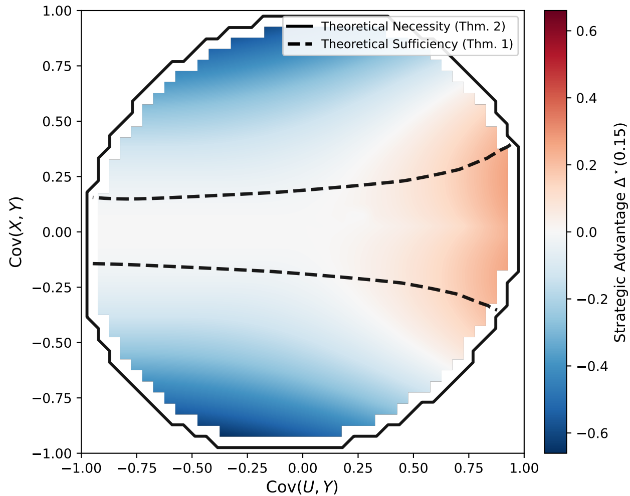
Strategic Advantage at Noise q = 0.15 ( \text{Cov}(X, U) = 0.1 )
