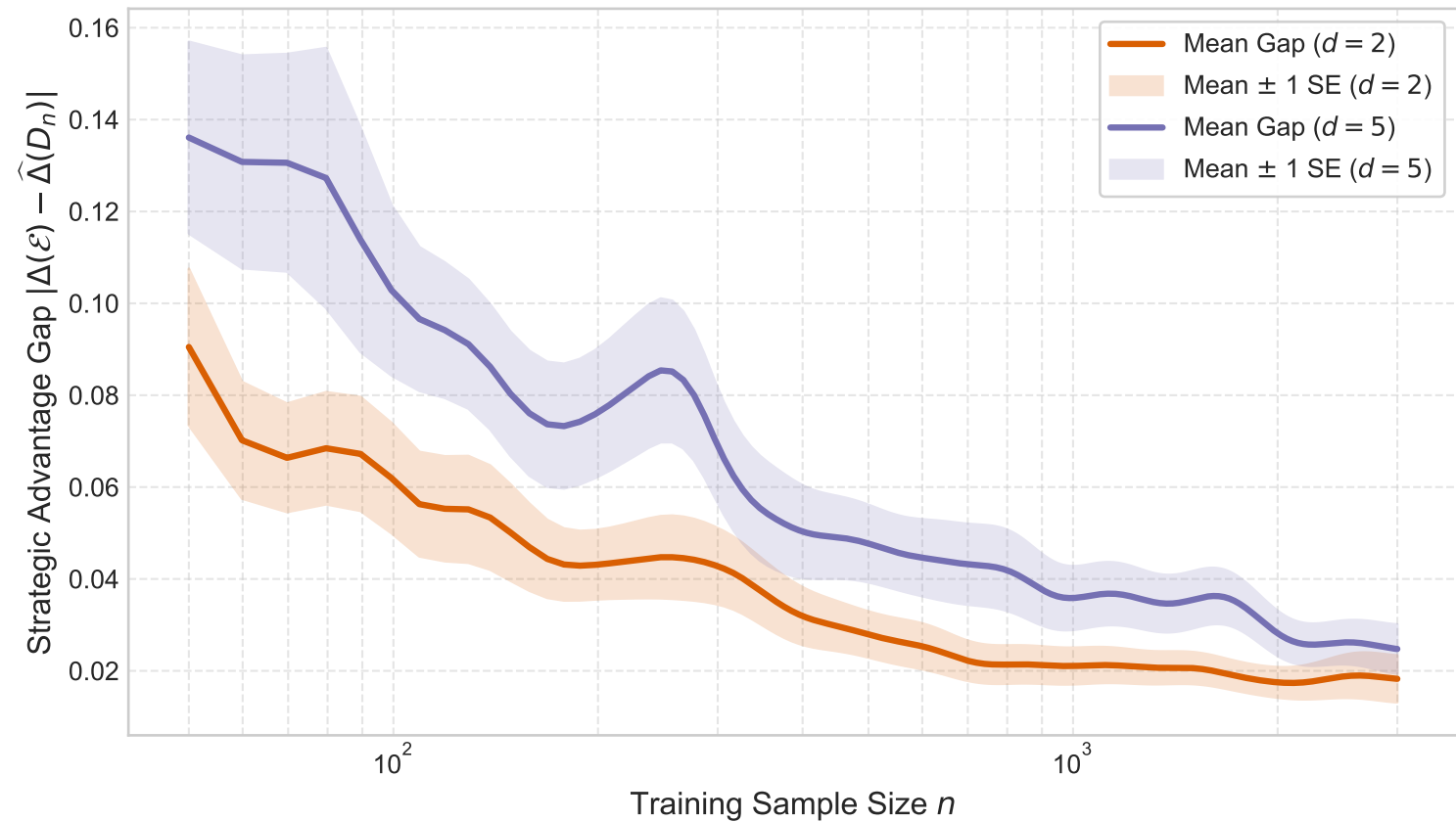
Strategic Advantage Generalization Gap vs. Sample Size ( q = 0.5 )
