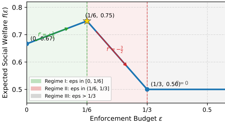
Analytical f(\varepsilon) : closed-form k = 2 example (\varepsilon^* = 1/6, \text{ peak welfare} = 3/4)
