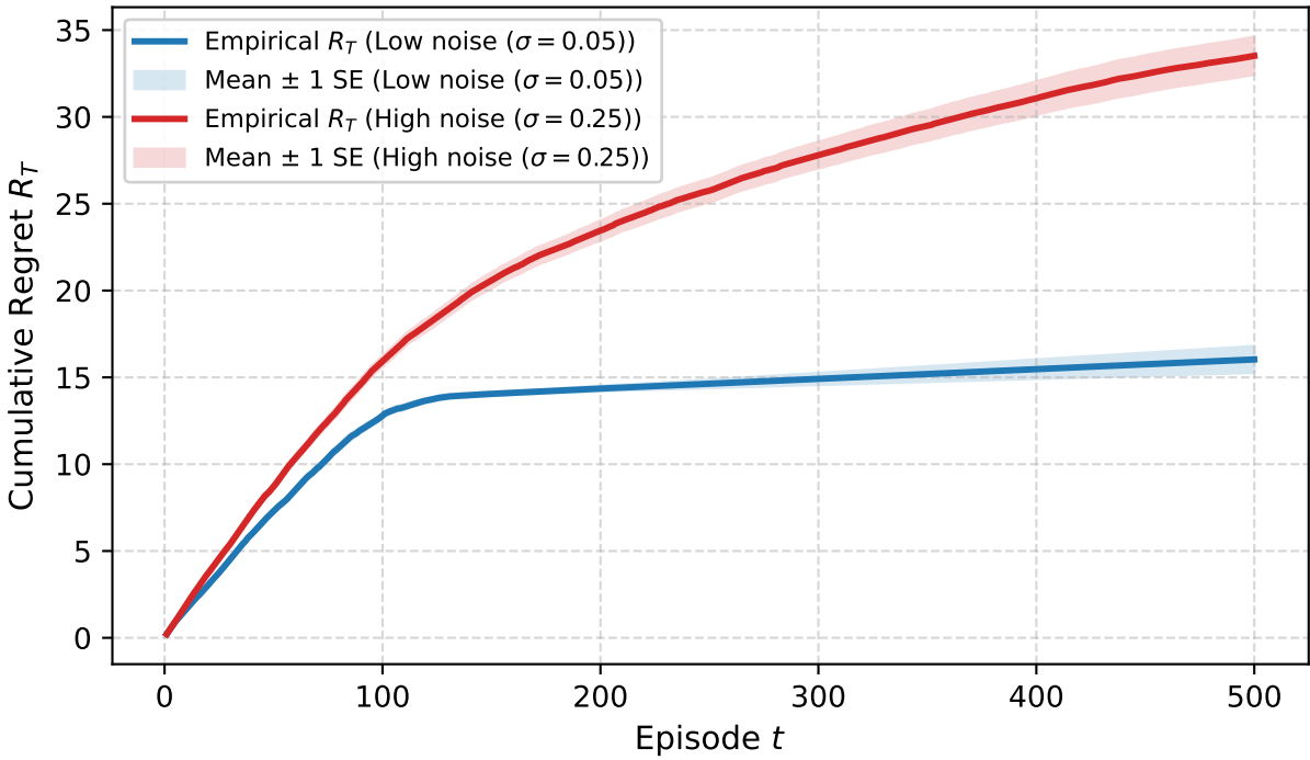
GP-TS Cumulative Regret R_T vs. Episodes T
