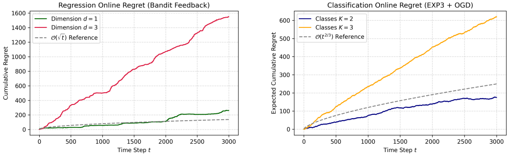
Fig. 4. Online expected cumulative regret curves under bandit feedback. Left: Regression regret under bandit OGD using one-point gradient estimates for d = 1 and d = 3 , showing O(\sqrt{t}) sublinear growth; Right: Classification regret under EXP3+OGD for K = 2 and K = 3 classes, confirming the sublinear O(t^{2/3}) regret bound.
