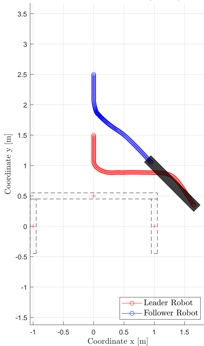
Leader-Follower Trajectory
