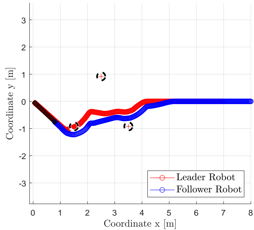
Leader-Follower Trajectory
