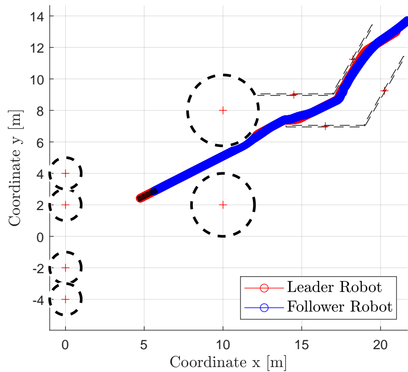
Leader-Follower Trajectory
