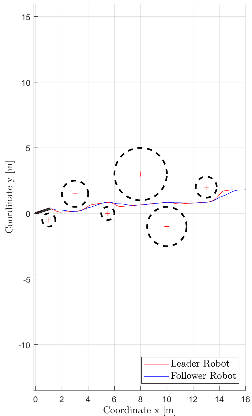
Leader-Follower Trajectory
