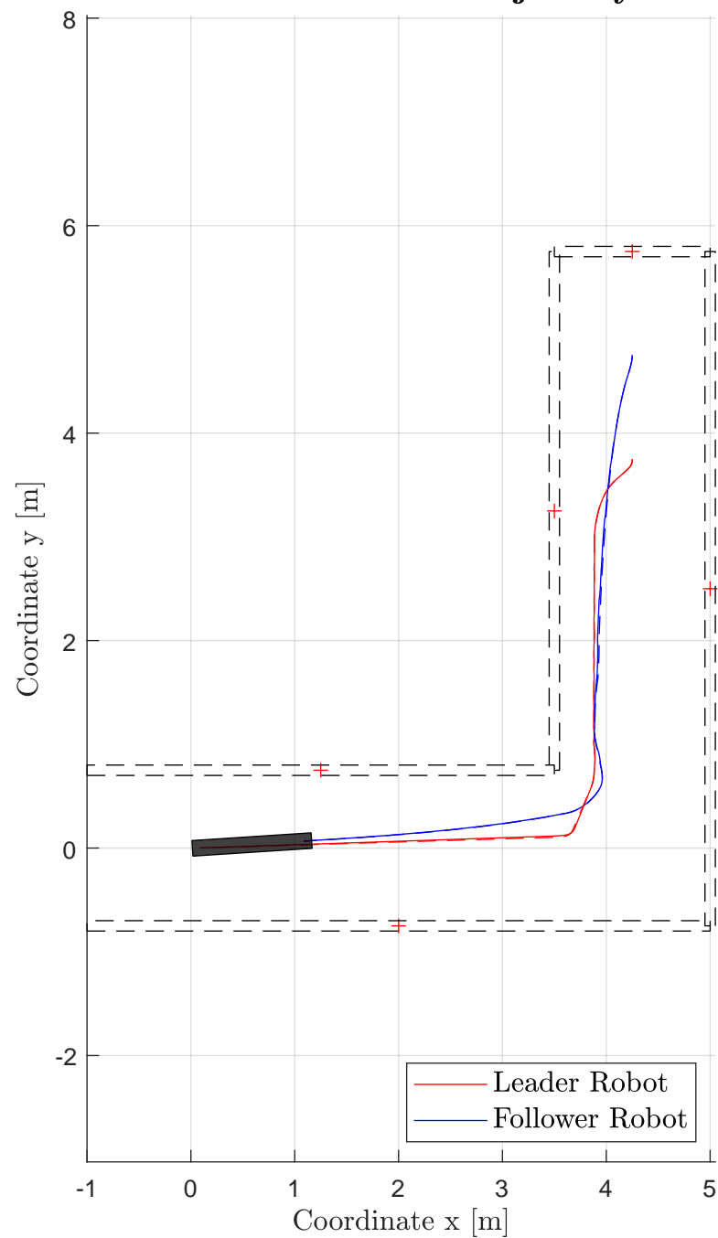
Leader-Follower Trajectory
