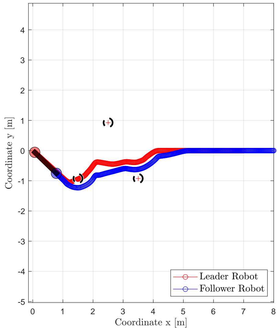
Leader-Follower Trajectory
