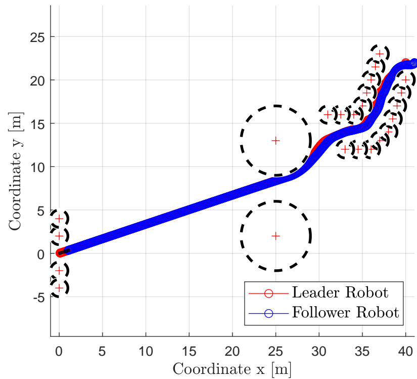
Leader-Follower Trajectory
