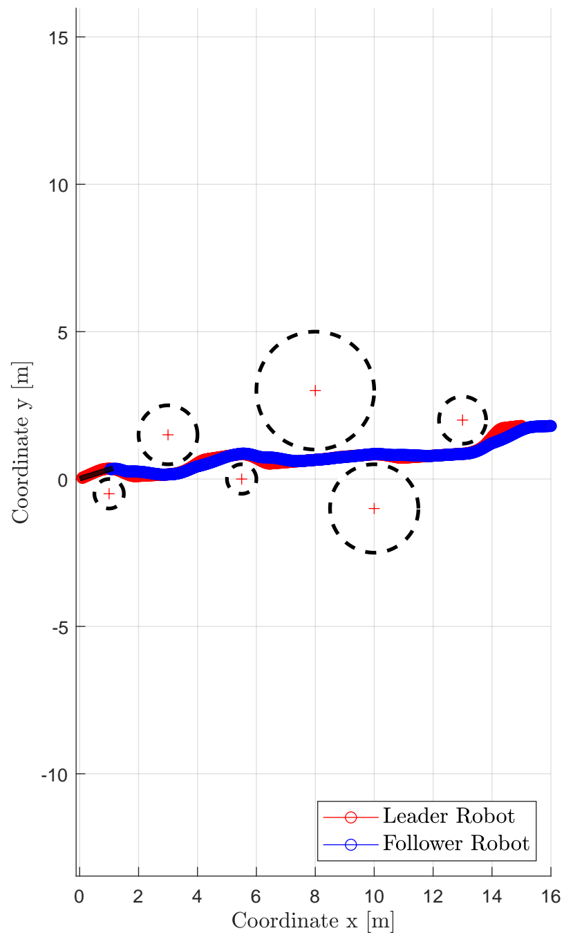
Leader-Follower Trajectory
