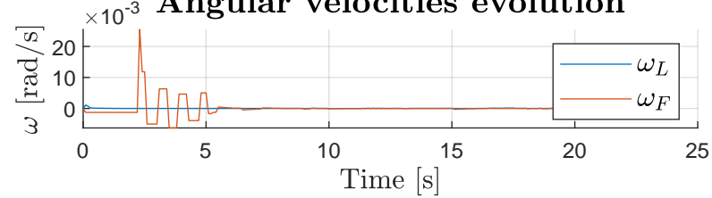
Angular velocities evolution
