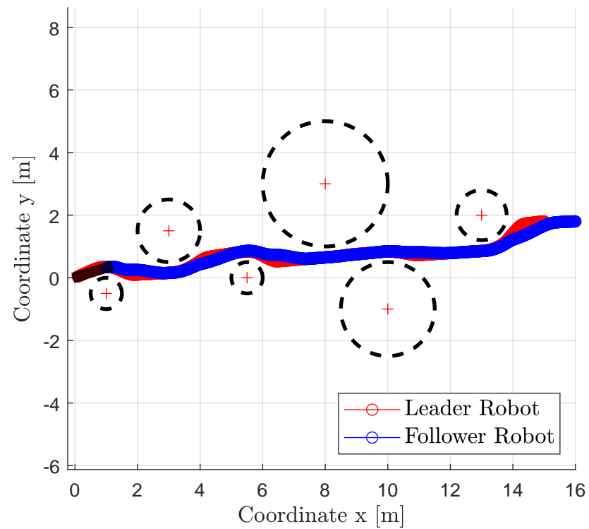
Leader-Follower Trajectory
