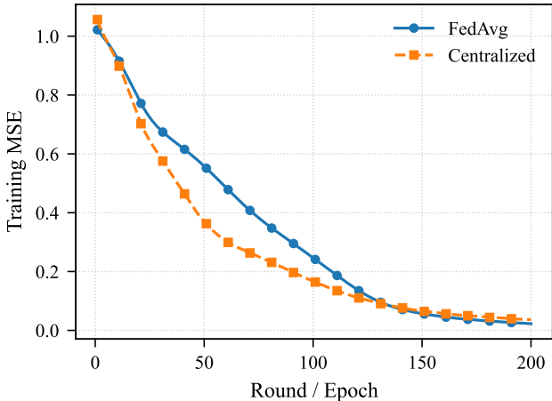
Training performance
