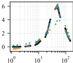
gfn1_test_impedance_dataset - Real parts (Y in S) Re(Y dd ) Re(Y dq ) Re(Y qd ) Re(Y qq ) Frequency Legend: TRUE (black solid line), Centralized (orange solid line), FedAvg (blue dashed line), Local-only (green dashed line)
