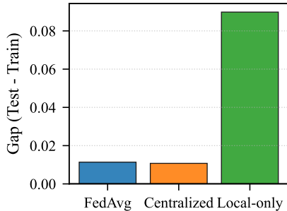
(c) Overfitting gap
