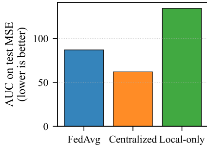
(b) Learning efficiency
