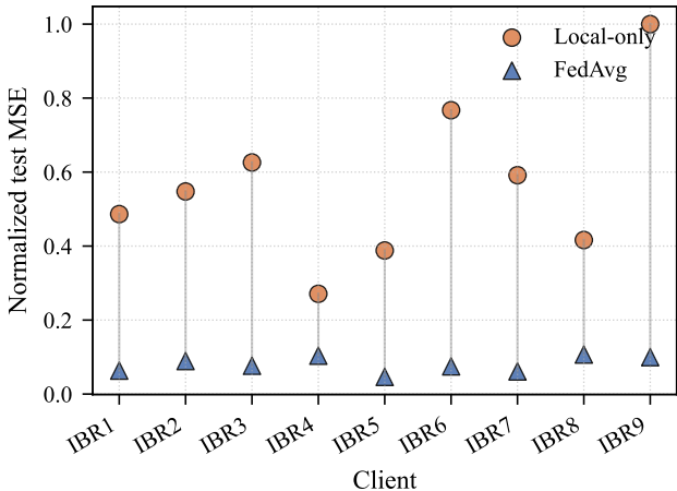
Normalized per-client performance
