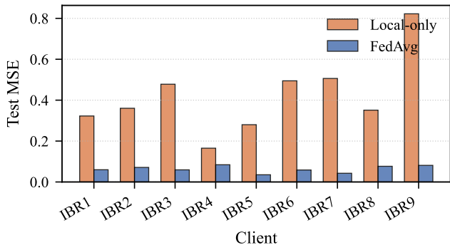
(a) Per-client test performance
