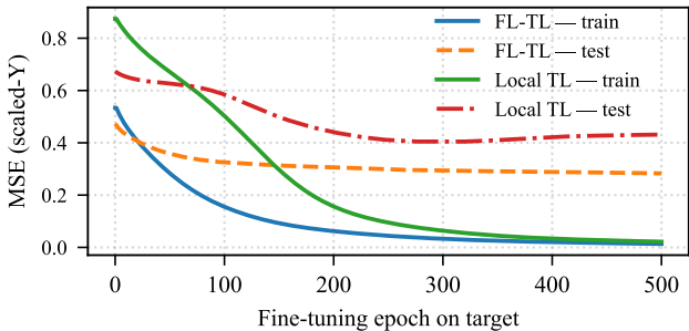
IBR1 — Overfitting check (train vs test, mean)
